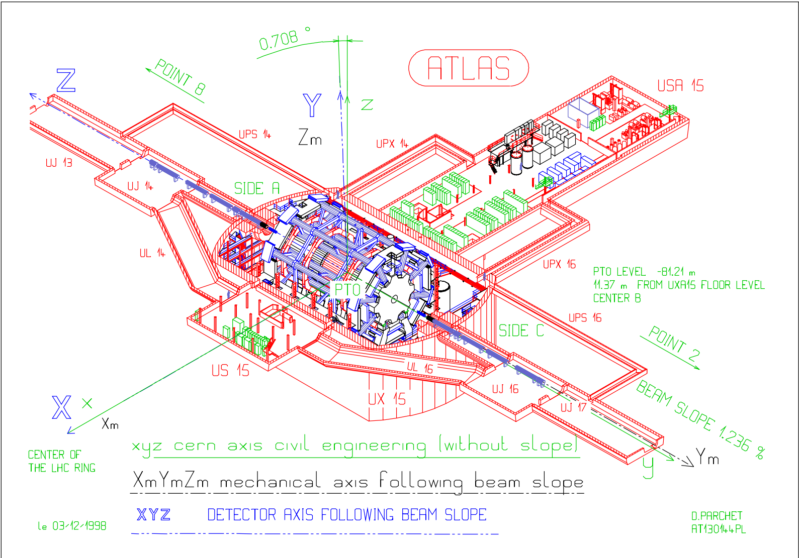
Figure 11-1 Graphical representation of the three axis systems used for ATLAS detector and experimental area.
