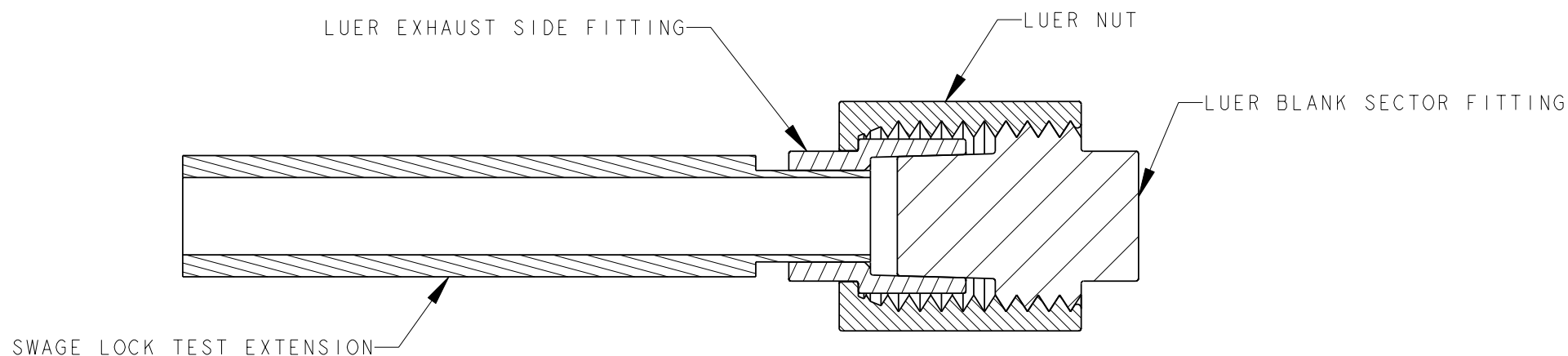
SECTION A - A LUER FITTING TEST SPECIMEN
