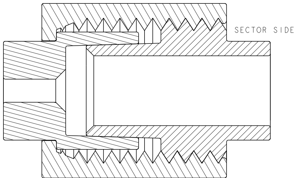
SECTION A - A SECTOR INLET JUNCTION
