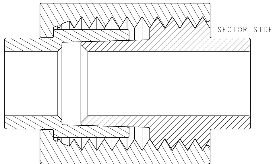
SECTION A - A SECTOR EXHAUST JUNCTION
