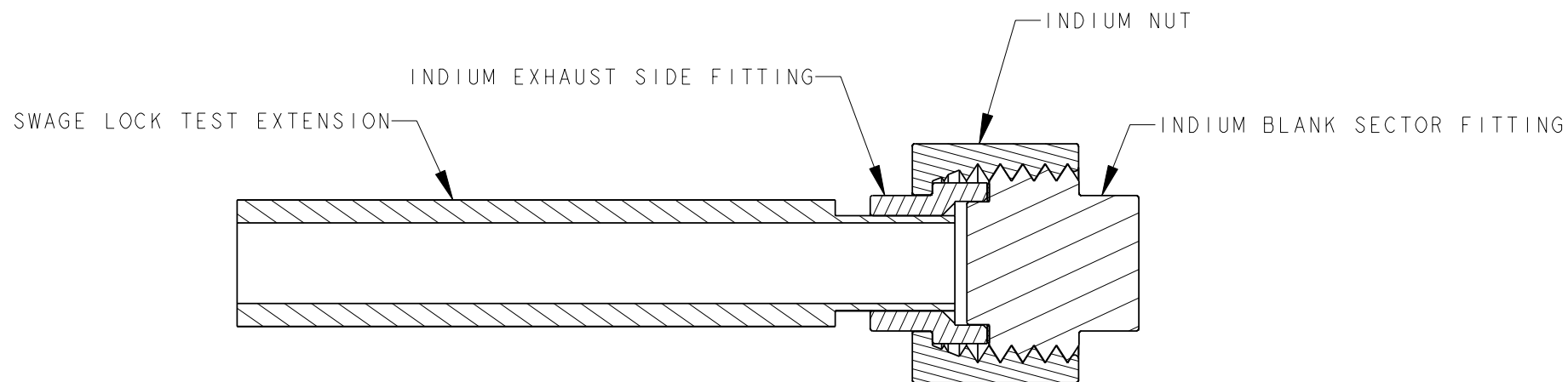
SECTION A - A INDIUM FITTING TEST SPECIMEN
