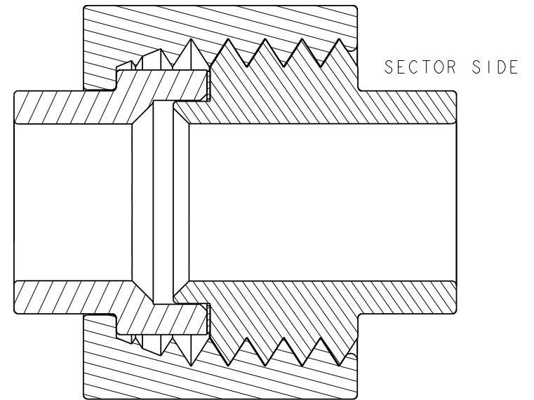
SECTION A - A SECTOR EXHAUST JUNCTION
