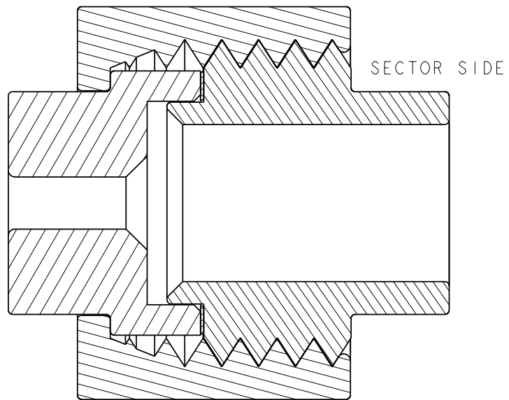
SECTION A - A SECTOR INLET JUNCTION
