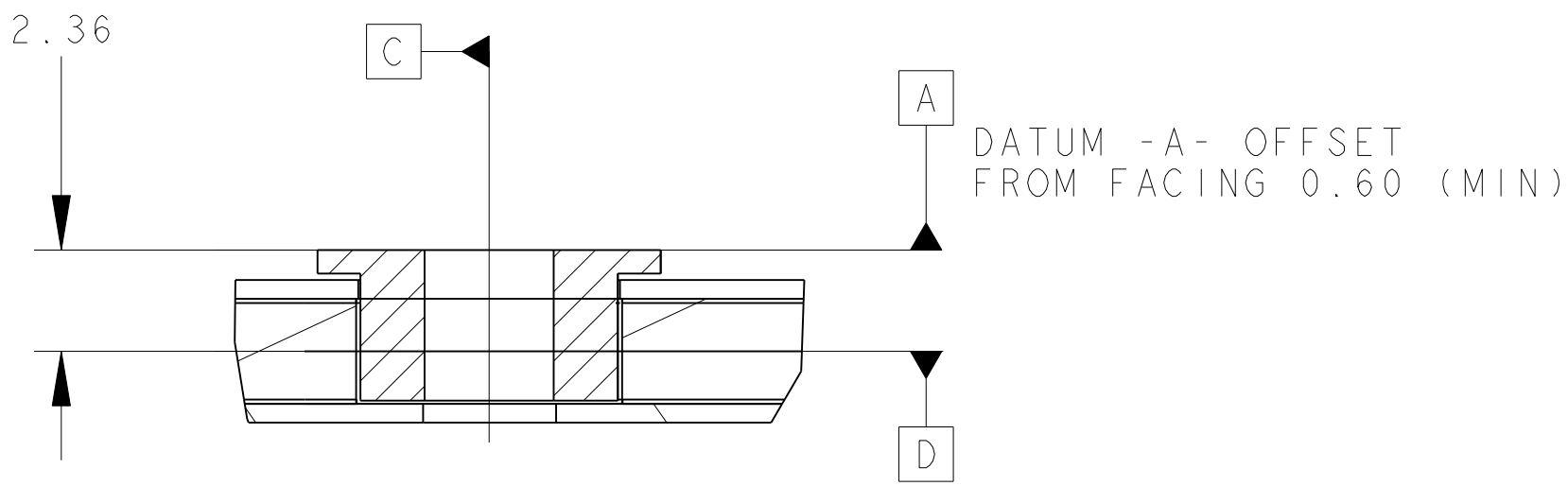
FACED_T-WASHER 6 / 1
