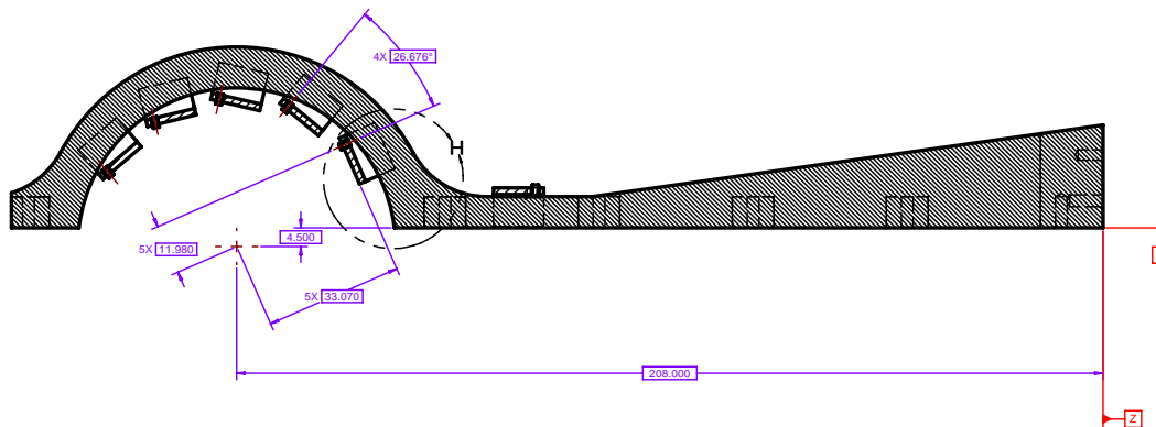
SECTION F-F
