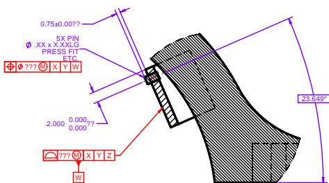
DETAIL H
