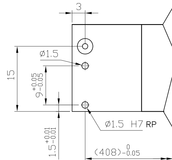
Detail D (2:1)
