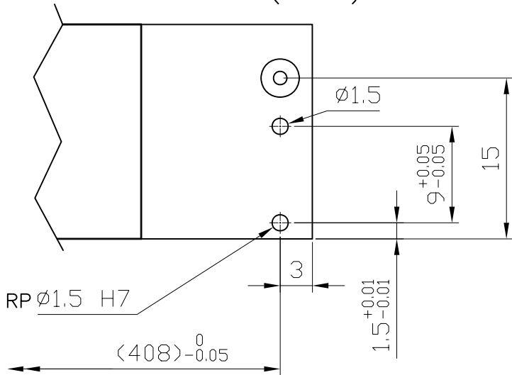
Detail D (2:1)
