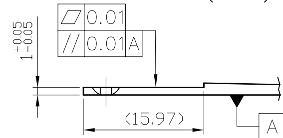
Detail B (2:1)
