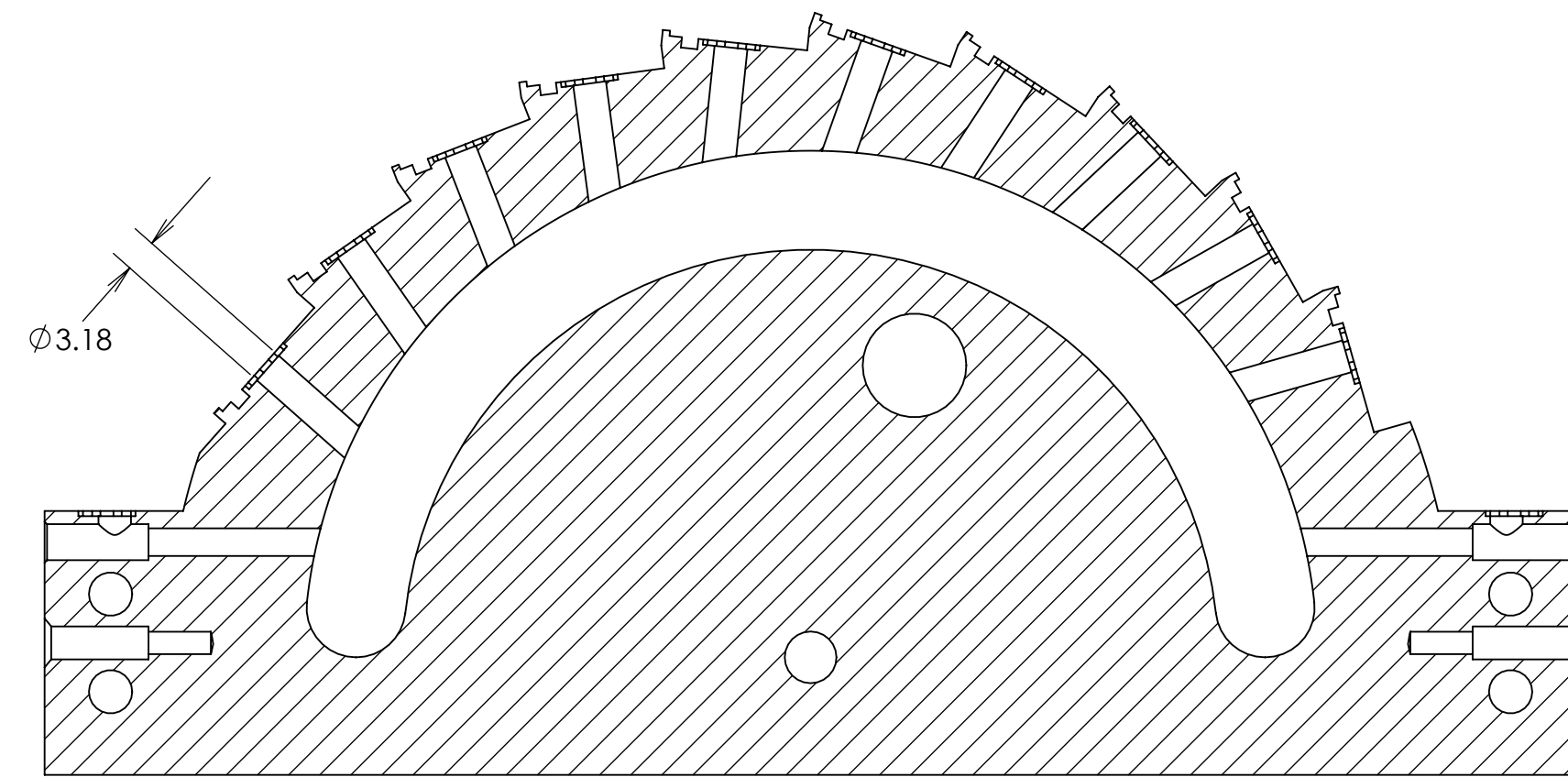
SECTION C-C
