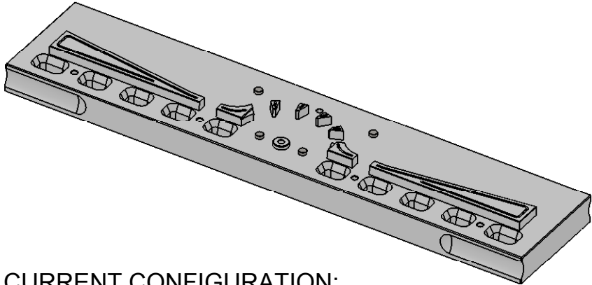
CURRENT CONFIGURATION: Base Plate With Pins Installed
