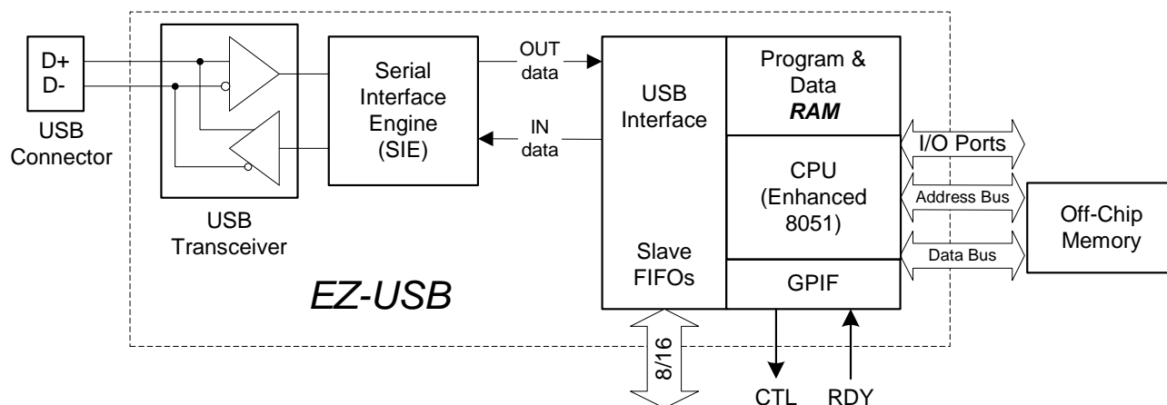
Figure 1-8. EZ-USB 128 Pin Package Simplified Block Diagram
