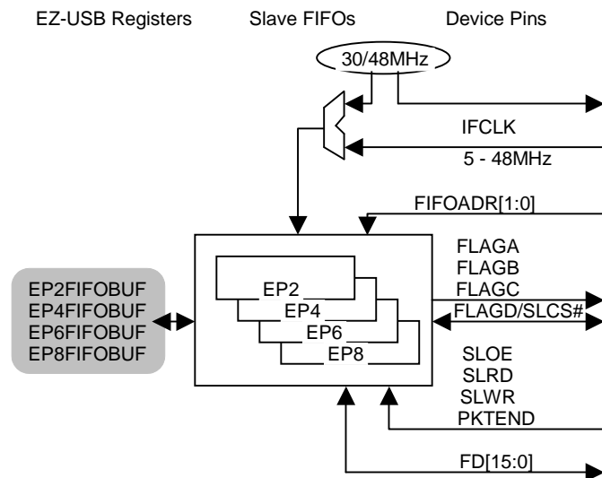
Figure 9-25. EPxFIFOBUF Registers
