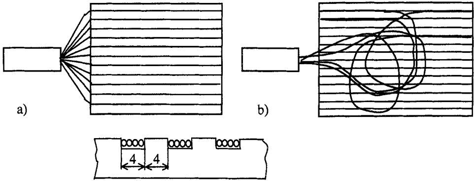
FIGURE 4. Design options for counters using flat grooves. a) one set of fibers in each groove; b) two set of fibers in each groove.
