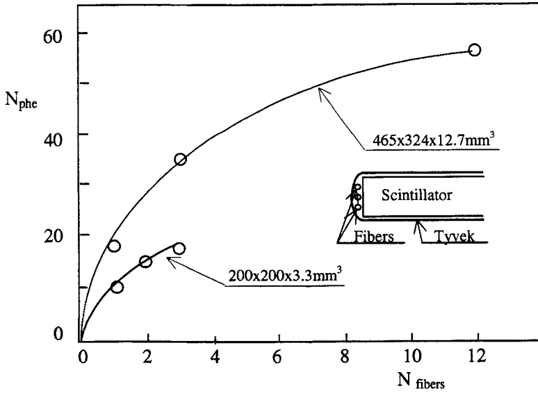
FIGURE 6. Number of photoelectrons versus number of fibers for design with fibers around the counters perimeter.
