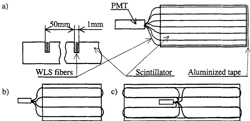
FIGURE 8. Deep grooves design. a) tested prototype; b), c) – design options.
