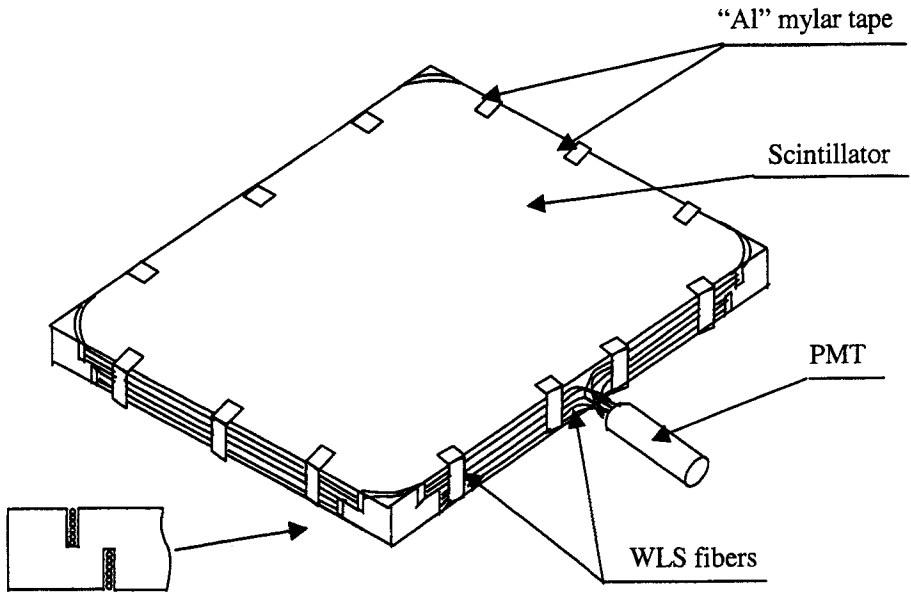
FIGURE 5. Design with fibers around the counter perimeter.
