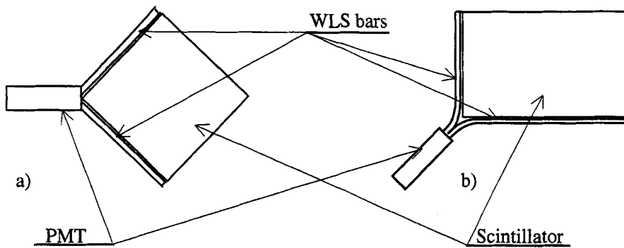
FIGURE 1. Counter design using WLS bars: a) cut at 45° bars; b) bent at 45° bars.
