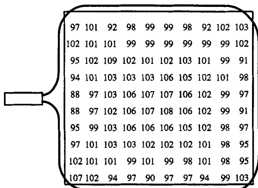
FIGURE 7. Uniformity of light response for counters using WLS fibers. Measurements used the radioactive source \text{Ru}^{106} . Counter 4, 200 \times 200 \times 3.3 \text{ mm}^3 , \sigma_I/I=4.2\% , I_{\text{max}}/I_{\text{min}}=1.21 .
