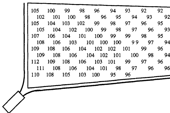
FIGURE 2. The uniformity of light response for counters using WLS bars. Measurements used the radioactive source \text{Ru}^{106} (current method). Counter 15, 465 \times 325 \times 12.7 \text{ mm}^3 , without masking. \sigma_I/I = 4.9\% , I_{\max}/I_{\min} = 1.22 .
