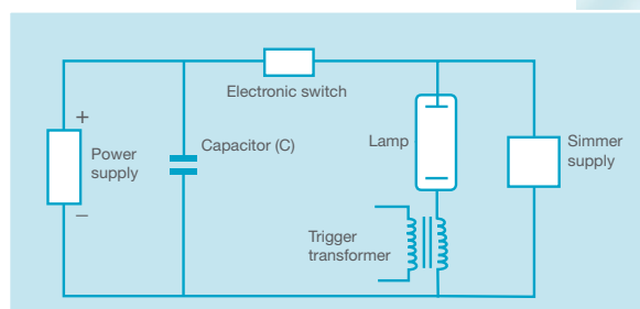
Fig.33 A basic drive circuit for square wave pulsing
