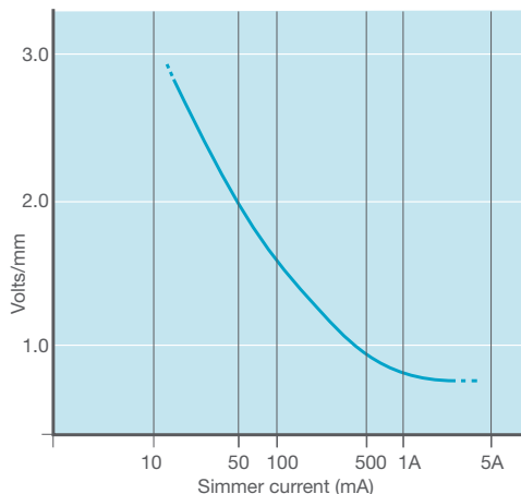
Fig.34 Generalised simmer curve
