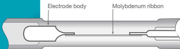
Fig.2 Ribbon Seal
