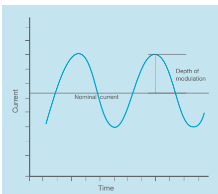
Fig.25 Quasi-CW operation
