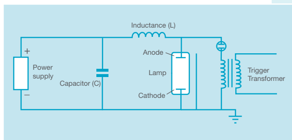
Fig.21 Typical parallel triggering circuit
