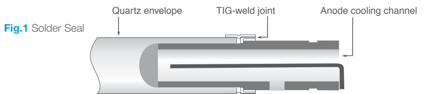
Fig.1 Solder Seal
