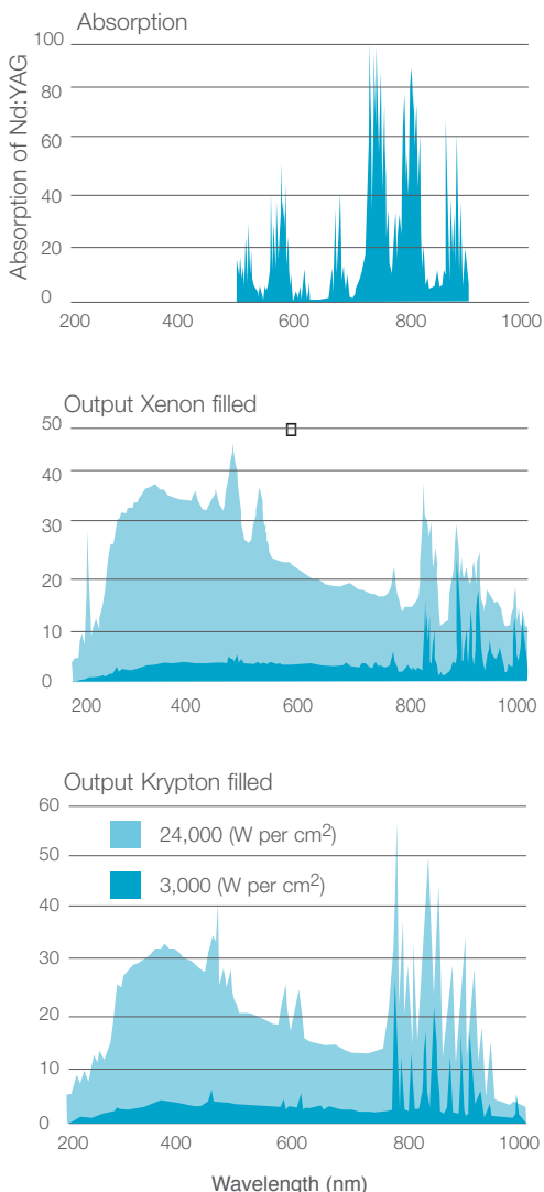
Fig.12 Spectral outputs of gas filled pulsed lamps
