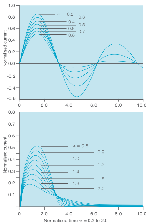
Fig.31 Current curves for different values of \alpha .
