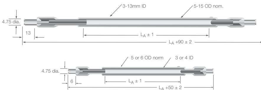
Fig.37 Air-cooled pulse lamp recommended physical dimensions (mm)
