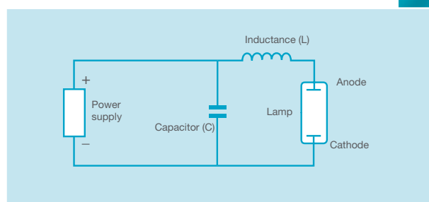
Fig.29 Simple pulsed lamp driving circuit
