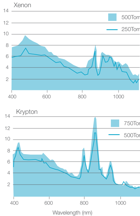
Fig.13 Variation of emission with cold fill pressure in pulsed lamps (4000W per cm 2 )
