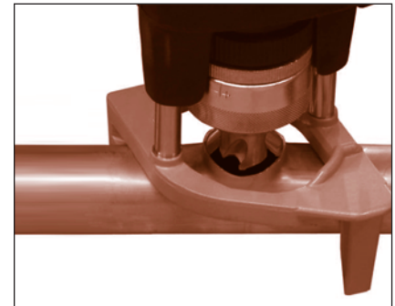
FIGURE 98: Forming the outlet
