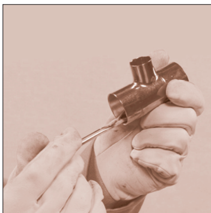
FIGURE 19: Fluxing: fitting
