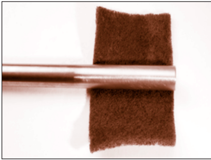
FIGURE 81: Cleaning the tube end
