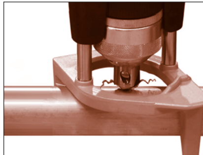
FIGURE 96: Positioning the drill tip and ensuring a snug fit of the support legs
