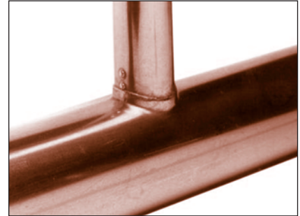
FIGURE 104: Finished joint
