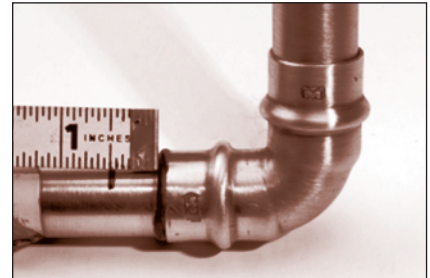
FIGURE 88: Ensuring proper insertion depth
