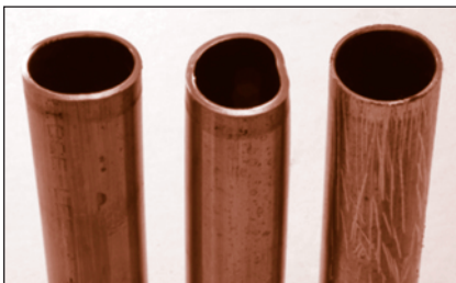
FIGURE 74: Check tube for imperfections
