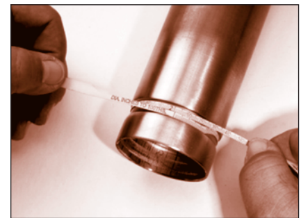
FIGURE 37: Grooved tube end
