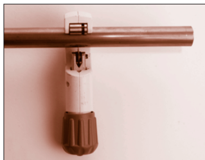
FIGURE 77: Cutting the tube square
