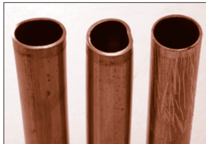
FIGURE 64: Ensure tube is clean, round and free of imperfections
