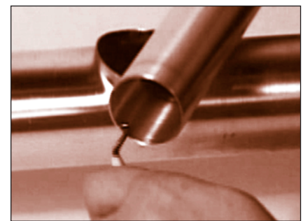
FIGURE 99: Reaming the branch tube end
