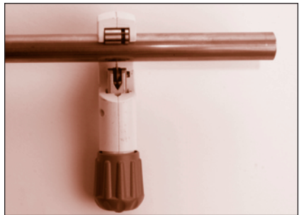
FIGURE 51: Cutting the tube square
