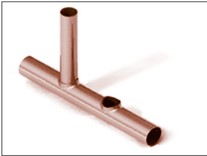
FIGURE 90: Mechanically formed extruded outlet requires only one brazed joint
