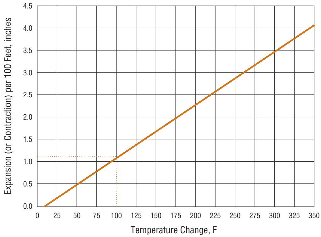
FIGURE 3. Expansion vs. Temperature Change for Copper Tube
