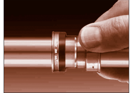
FIGURE 73: Completed installation of a push-connect joint
