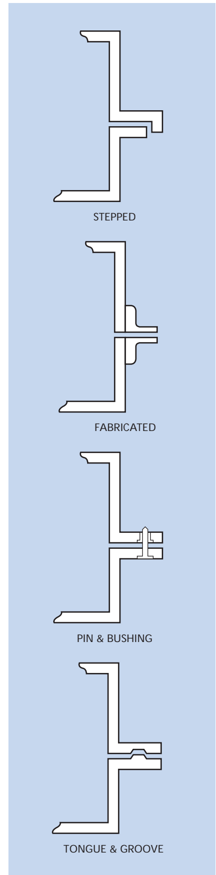
Figure 5. Parting Lines
