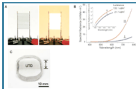
Fig. 3. Application as a broadband source of polarized incandescent light and for the microwave welding of plastics. (A) Photograph showing a free-standing undensified MWNT sheet (16 mm by 22 mm) used as a planar incandescent light source that emits polarized radiation. The background color of the unheated sheet (left) and the incandescent sheet (right) differs because of reflected incandescent light from a white paper sheet that is behind the light source. (B) Spectral radiance in directions parallel to (||) and perpendicular to (⊥) the draw direction of an as-drawn undensified MWNT sheet after an added inelastic stretch in the initial draw direction of 2.5%. The luminance polarized parallel to the sheet draw direction for the indicated spectral range is 6.1 times higher than for the perpendicularly polarized luminance, which corresponds to a polarization factor of 0.72. The inset shows these data on a semilogarithmic scale. Underlying solid lines (largely obscured by coincidence with the data points) are data fits assuming black-body radiation with T = 1410 K. (C) Photograph of two 5-mm-thick Plexiglas plates that have been welded together by microwave-induced heating of an as-drawn MWNT sheet strip that was sandwiched between these plates. The nanotube sheet strip at the welded interface (see arrow for vertical extension) remains oriented, highly conducting, and transparent, as indicated by the visibility of "UTD" printed on an underlying paper sheet. [View Larger Version of this Image (36K GIF file)]
