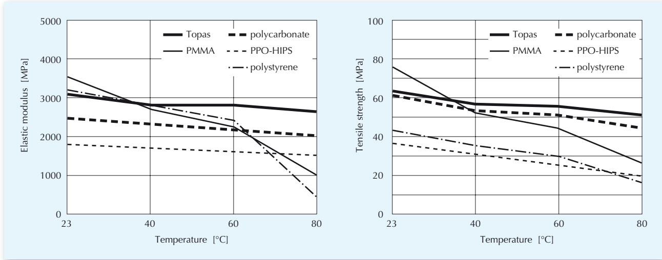
Fig. 3 and 4: Effect of temperature on the elastic modulus and tensile strength of Topas COC resin compared with other transparent amorphous thermoplastics. This is valid with good approximation for grades 5013, 6013, 6015 and 6017
