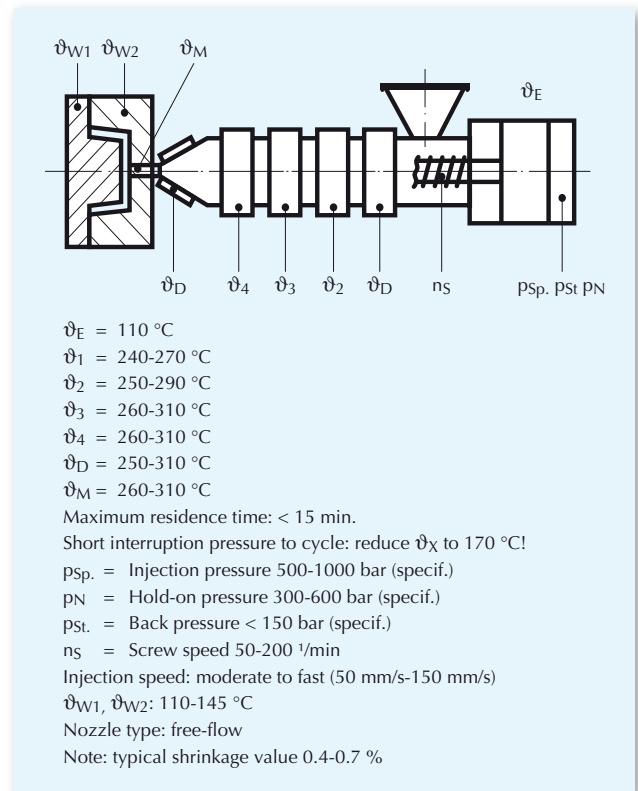
Fig. 13: Processing conditions for Topas 6015
