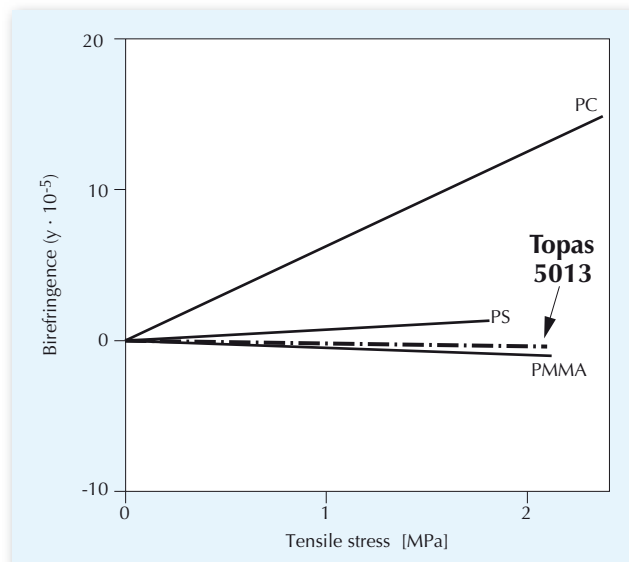
Fig. 10: Stress birefringence of various plastics (birefringence as a function of tensile stress)
