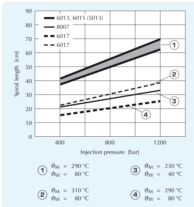
Fig. 12: Spiral flow length of Topas grades with different glass transition temperatures as a function of pressure (2 mm-thick test spiral). The processing parameters ( \vartheta_M = melt temperature, \vartheta_W = mold wall temperature) were matched to the glass transition temperature of the Topas grades
