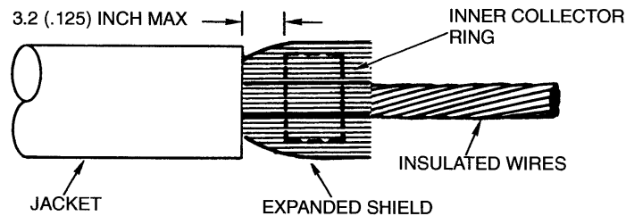
B. PLACEMENT OF COLLECTOR RING FOR OVERALL SHIELD
