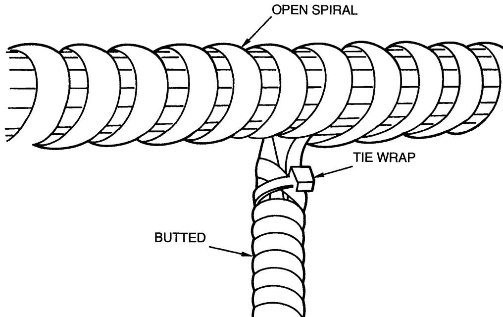
Figure 9-11. Spiral Wrap Sleeving
