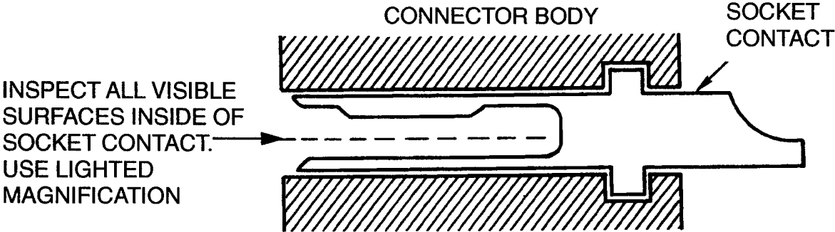
Figure 15-1. Visual Examination Inside the Socket Contact for Flux Residue
