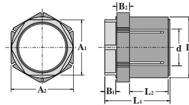
Trantorque GT
