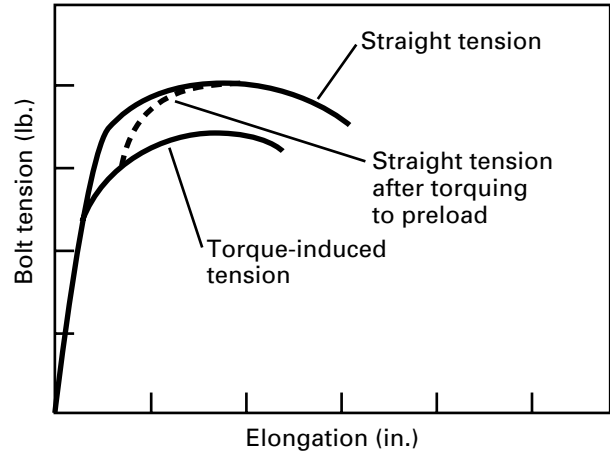
Fig. 13 Torque/Tension Relationship
