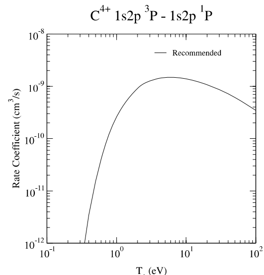
Graph 42: Rate coefficient for electron-impact excitation.
