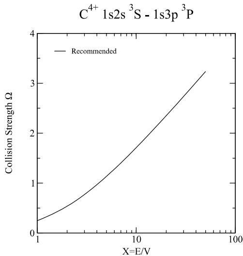
Graph 35: Collision strength for electron-impact excitation.
