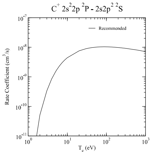
Graph 98: Rate coefficient for electron-impact excitation.
