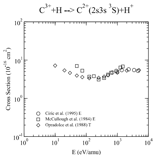
Graph 169: Cross section for charge exchange.
