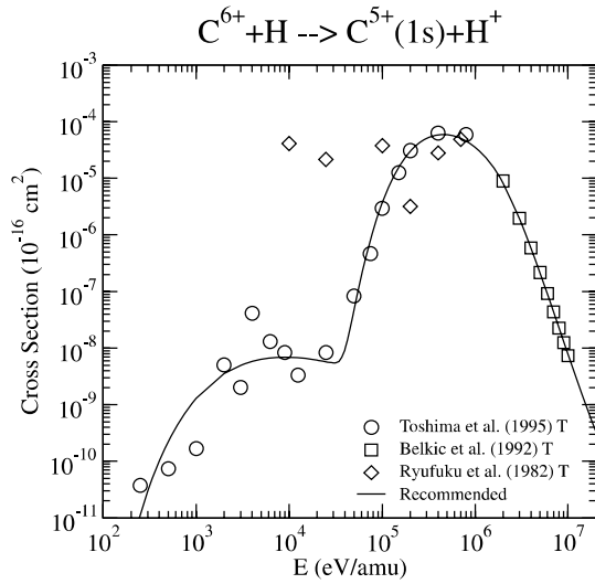
Graph 139: Cross section for charge exchange.
