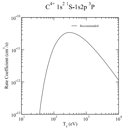
Graph 22: Rate coefficient for electron-impact excitation.
