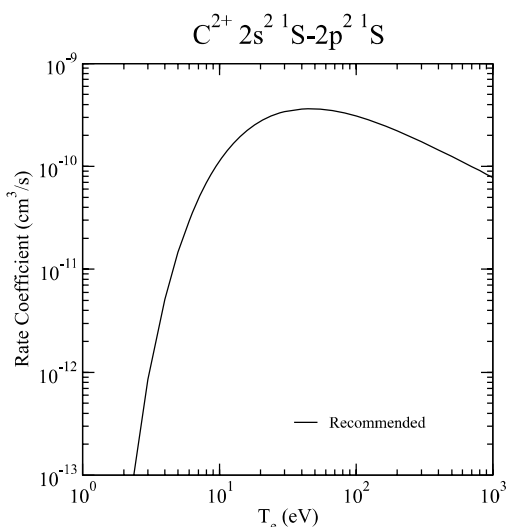
Graph 70: Rate coefficient for electron-impact excitation.
