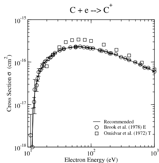
Graph 137: Cross section for electron-impact ionization.
