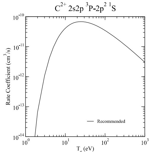
Graph 80: Rate coefficient for electron-impact excitation.
