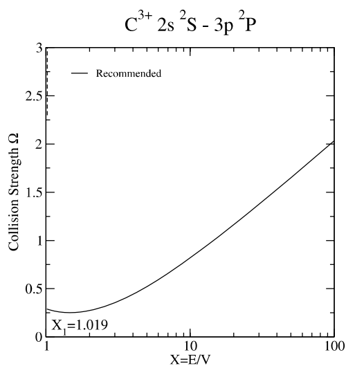
Graph 49: Collision strength for electron-impact excitation.
