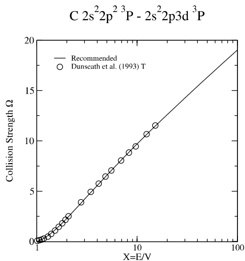
Graph 123: Collision strength for electron-impact excitation.
