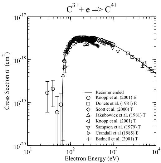
Graph 129: Cross section for electron-impact ionization.
