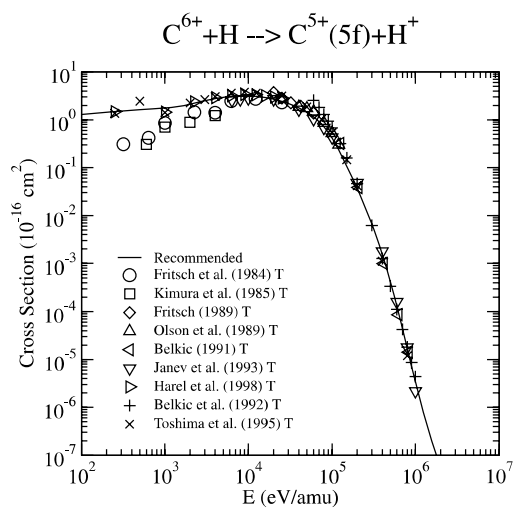
Graph 155: Cross section for charge exchange.
