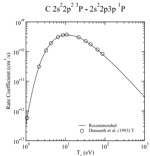
Graph 120: Rate coefficient for electron-impact excitation.
