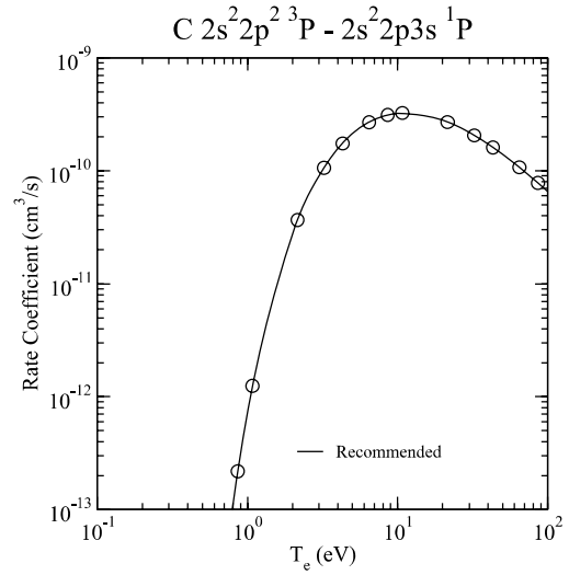
Graph 116: Rate coefficient for electron-impact excitation.
