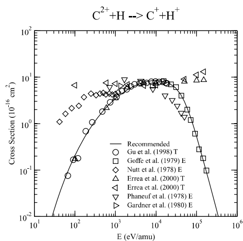
Graph 173: Cross section for charge exchange.
