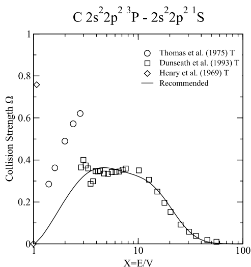
Graph 109: Collision strength for electron-impact excitation.
