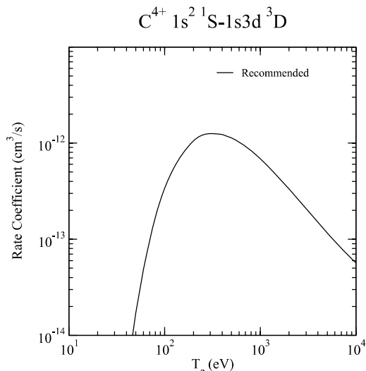
Graph 26: Rate coefficient for electron-impact excitation.
