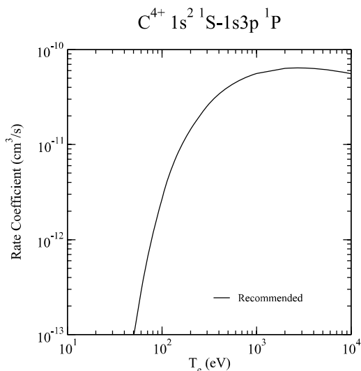
Graph 28: Rate coefficient for electron-impact excitation.
