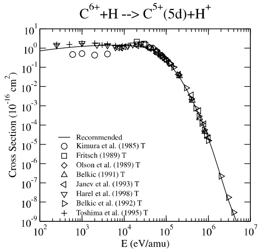
Graph 154: Cross section for charge exchange.
