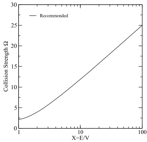
Graph 105: Collision strength for electron-impact excitation.
