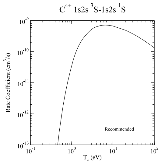
Graph 30: Rate coefficient for electron-impact excitation.
