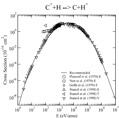
Graph 174: Cross section for charge exchange.
