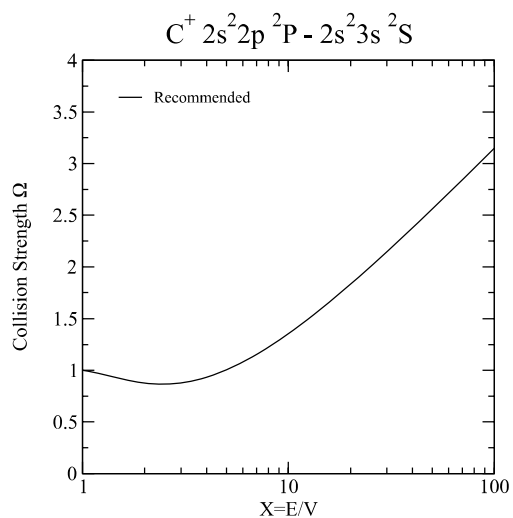
Graph 101: Collision strength for electron-impact excitation.
