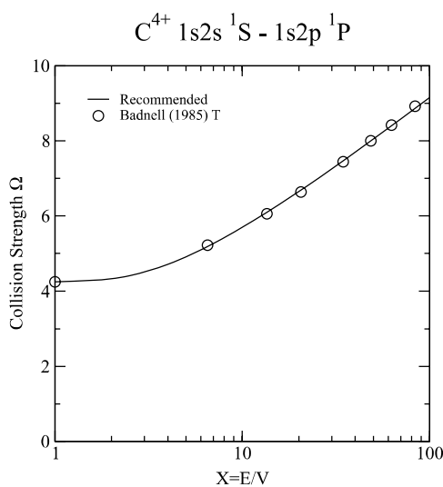
Graph 39: Collision strength for electron-impact excitation.
