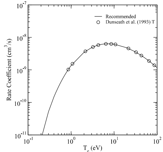
Graph 108: Rate coefficient for electron-impact excitation.
