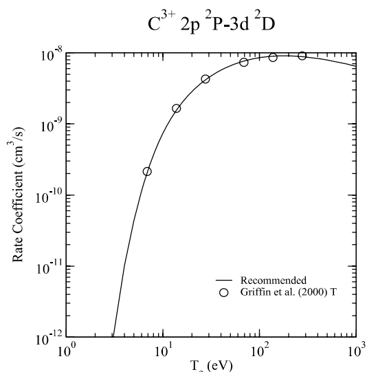
Graph 58: Rate coefficient for electron-impact excitation.
