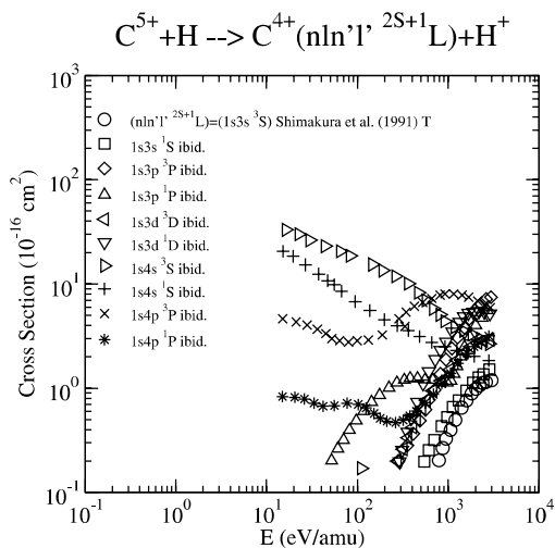
Graph 159: Cross section for charge exchange.
