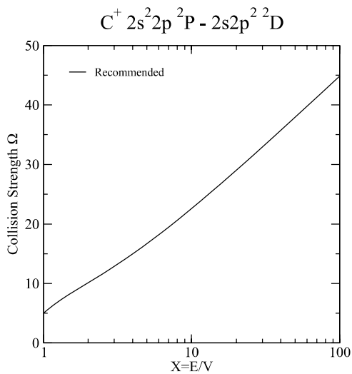
Graph 95: Collision strength for electron-impact excitation.
