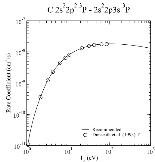
Graph 114: Rate coefficient for electron-impact excitation.
