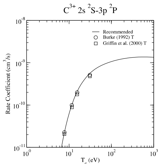
Graph 50: Rate coefficient for electron-impact excitation.
