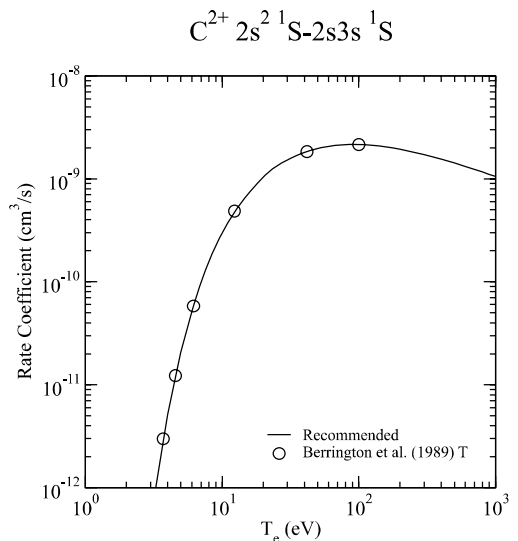
Graph 72: Rate coefficient for electron-impact excitation.
