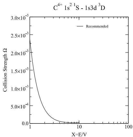
Graph 25: Collision strength for electron-impact excitation.
