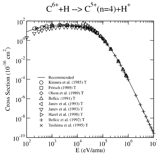
Graph 151: Cross section for charge exchange.
