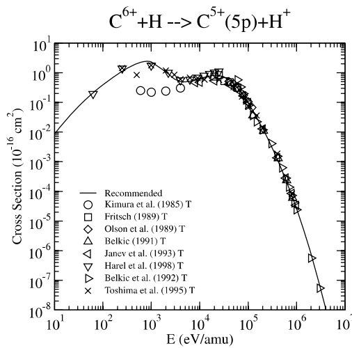
Graph 153: Cross section for charge exchange.
