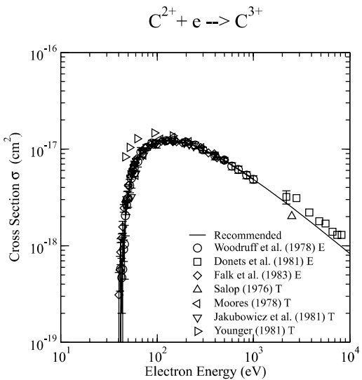
Graph 131: Cross section for electron-impact ionization.
