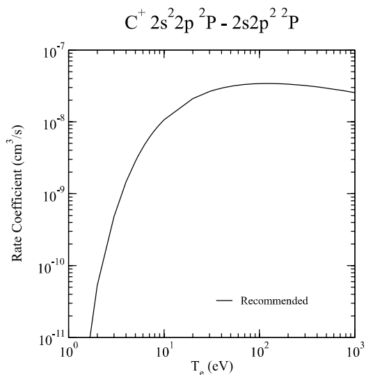
Graph 100: Rate coefficient for electron-impact excitation.
