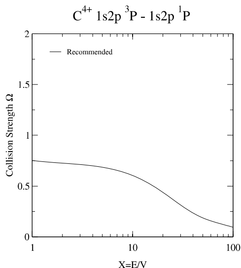
Graph 41: Collision strength for electron-impact excitation.
