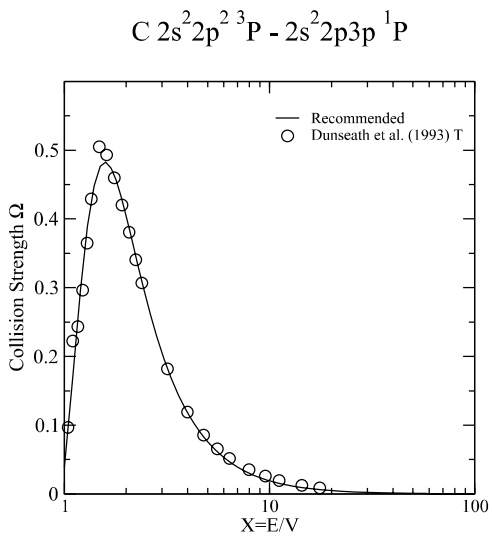
Graph 119: Collision strength for electron-impact excitation.
