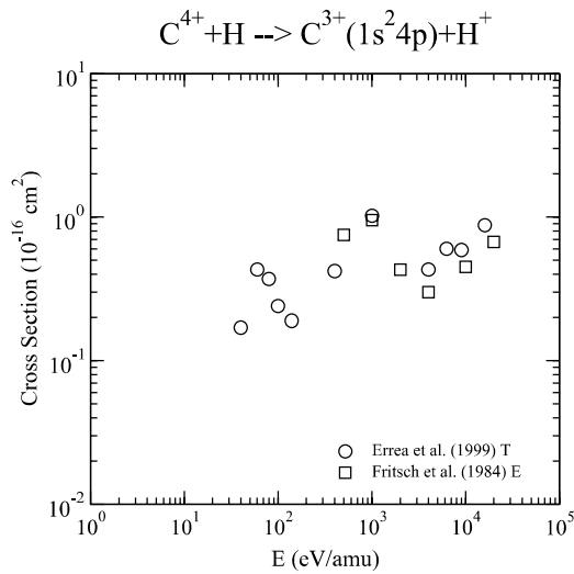
Graph 165: Cross section for charge exchange.
