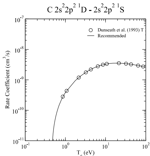
Graph 112: Rate coefficient for electron-impact excitation.
