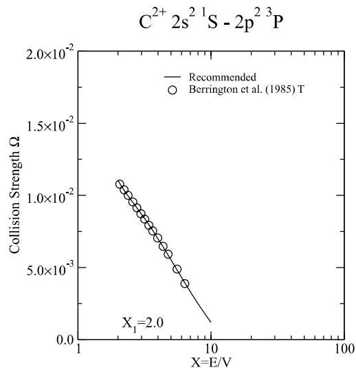
Graph 65: Collision strength for electron-impact excitation.
