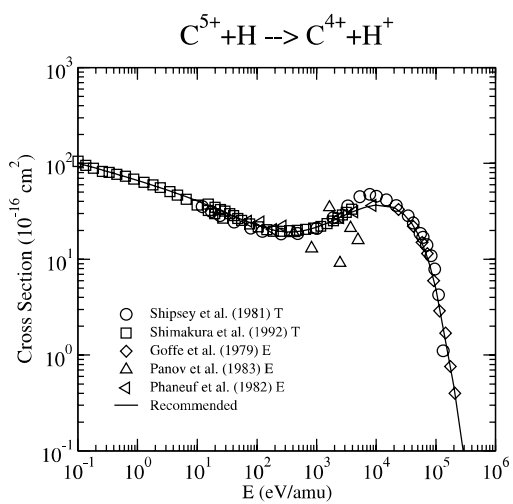
Graph 160: Cross section for charge exchange.
