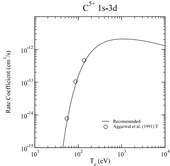
Graph 10: Rate coefficient for electron-impact excitation.
