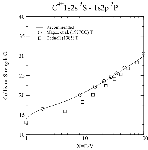
Graph 31: Collision strength for electron-impact excitation.
