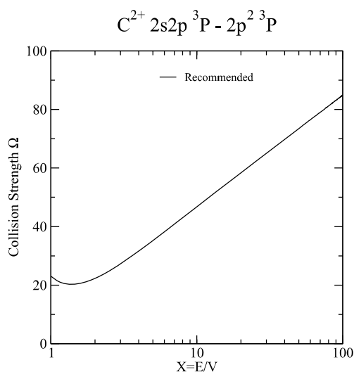
Graph 75: Collision strength for electron-impact excitation.
