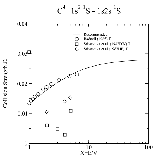
Graph 19: Collision strength for electron-impact excitation.
