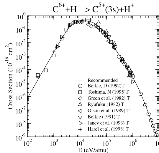
Graph 143: Cross section for charge exchange.
