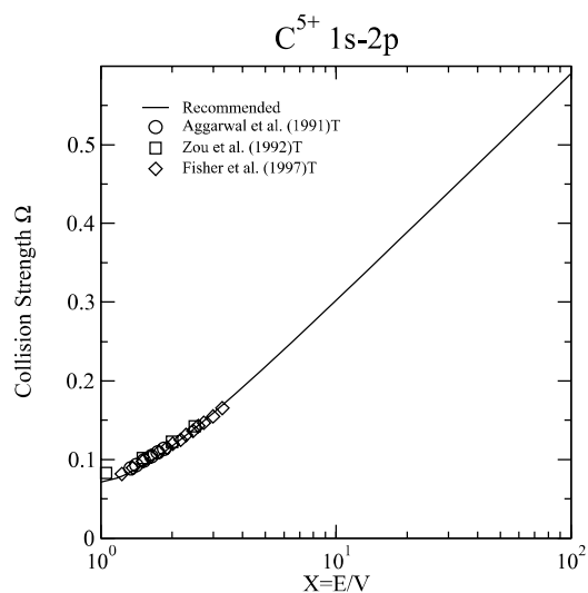
Graph 3: Collision strength for electron-impact excitation.
