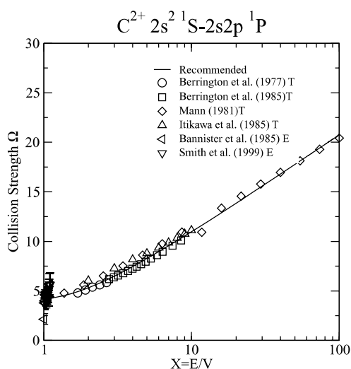
Graph 63: Collision strength for electron-impact excitation.
