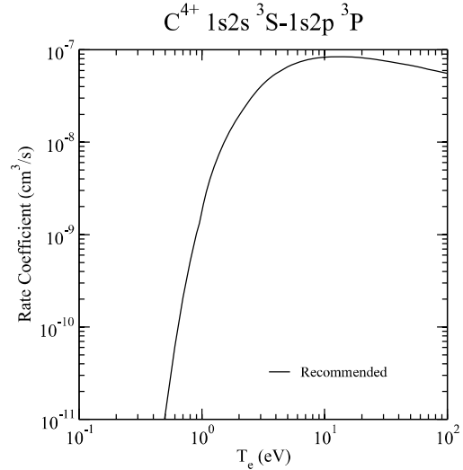
Graph 32: Rate coefficient for electron-impact excitation.
