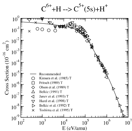
Graph 152: Cross section for charge exchange.
