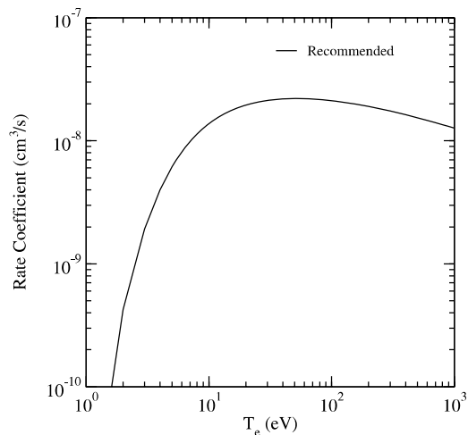
Graph 86: Rate coefficient for electron-impact excitation.
