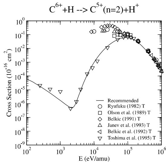
Graph 142: Cross section for charge exchange.
