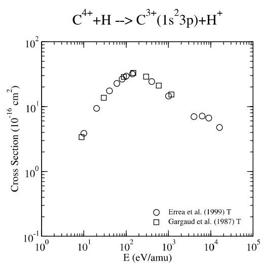
Graph 162: Cross section for charge exchange.
