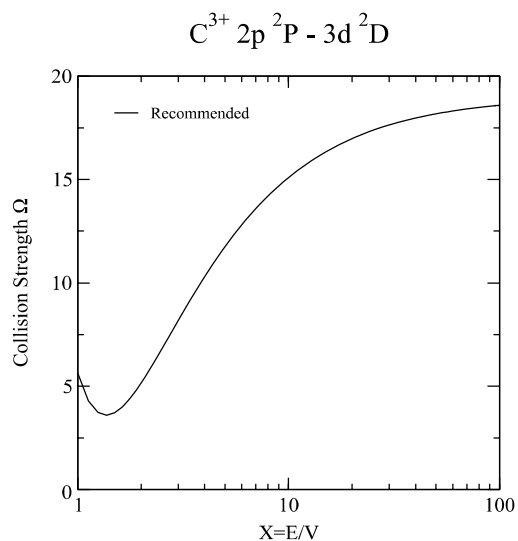
Graph 57: Collision strength for electron-impact excitation.
