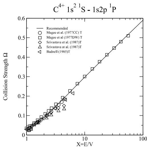
Graph 23: Collision strength for electron-impact excitation.
