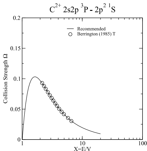
Graph 79: Collision strength for electron-impact excitation.
