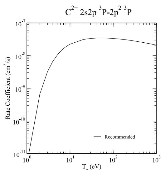
Graph 76: Rate coefficient for electron-impact excitation.
