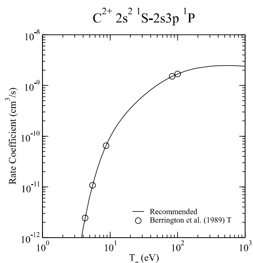
Graph 74: Rate coefficient for electron-impact excitation.
