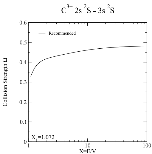
Graph 47: Collision strength for electron-impact excitation.
