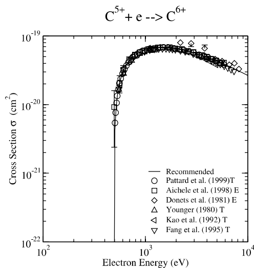
Graph 125: Cross section for electron-impact ionization.
