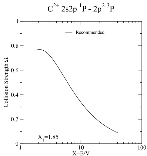
Graph 81: Collision strength for electron-impact excitation.
