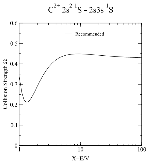
Graph 71: Collision strength for electron-impact excitation.
