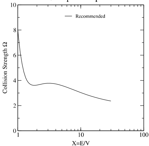
Graph 87: Collision strength for electron-impact excitation.
