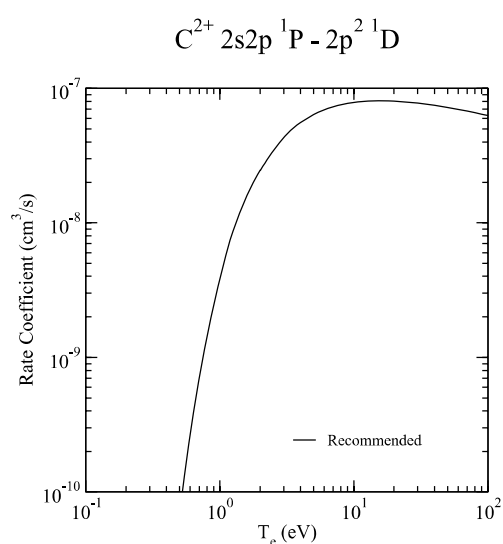
Graph 84: Rate coefficient for electron-impact excitation.
