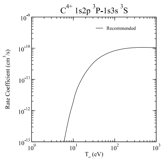
Graph 44: Rate coefficient for electron-impact excitation.
