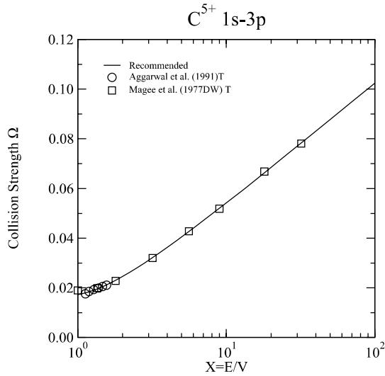
Graph 7: Collision strength for electron-impact excitation.
