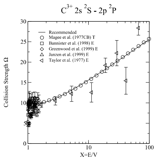
Graph 45: Collision strength for electron-impact excitation.
