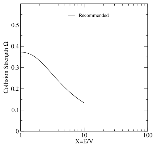
Graph 89: Collision strength for electron-impact excitation.
