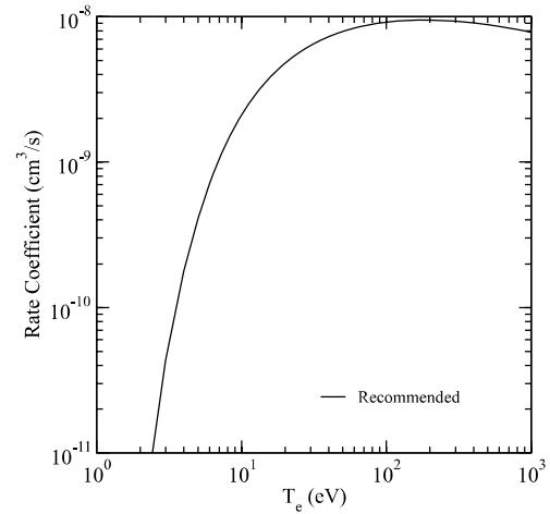
Graph 106: Rate coefficient for electron-impact excitation.
