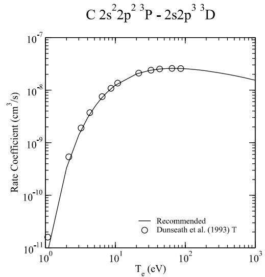
Graph 118: Rate coefficient for electron-impact excitation.
