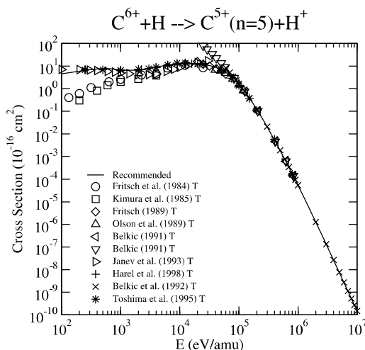
Graph 157: Cross section for charge exchange.
