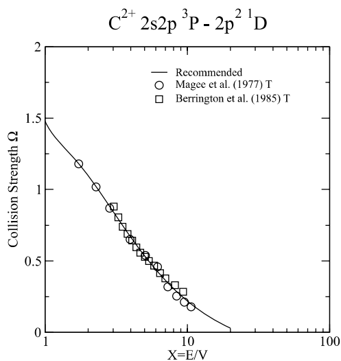
Graph 77: Collision strength for electron-impact excitation.
