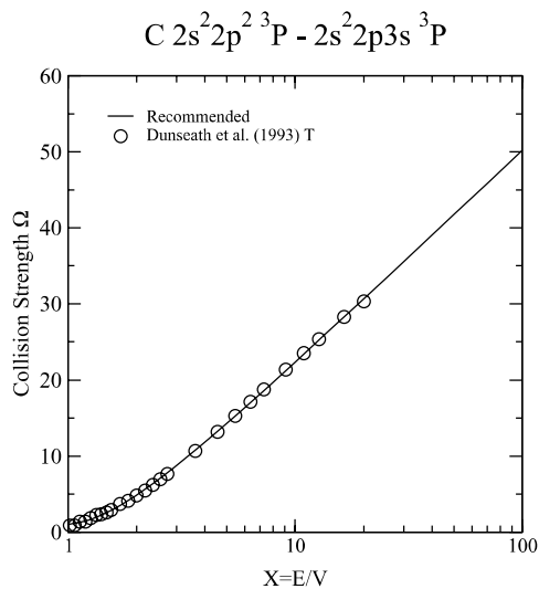
Graph 113: Collision strength for electron-impact excitation.
