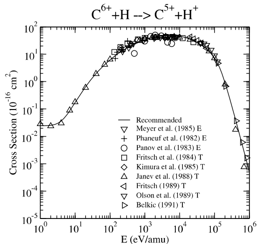
Graph 158: Cross section for charge exchange.
