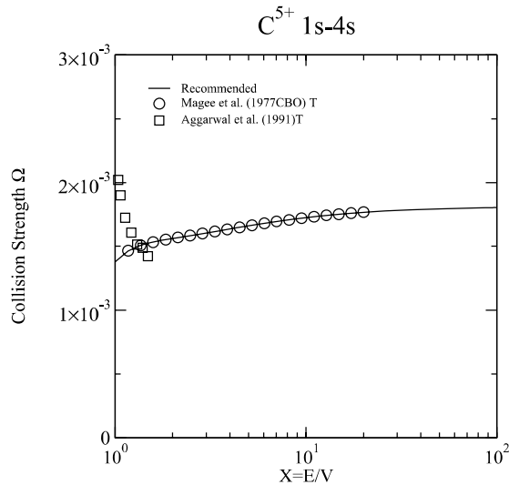
Graph 11: Collision strength for electron-impact excitation.
