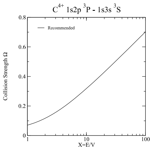
Graph 43: Collision strength for electron-impact excitation.
