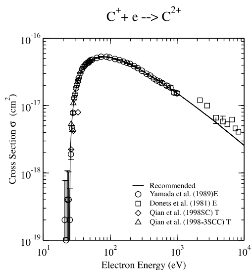
Graph 133: Cross section for electron-impact ionization.
