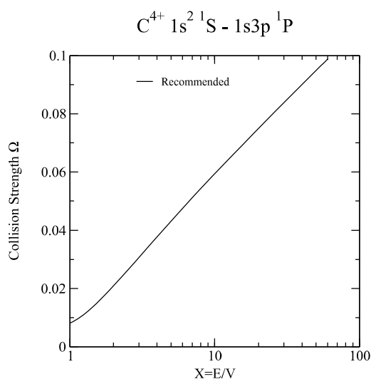
Graph 27: Collision strength for electron-impact excitation.
