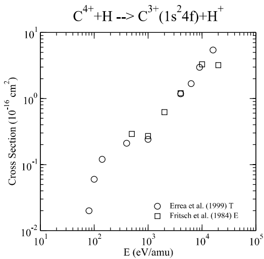
Graph 167: Cross section for charge exchange.
