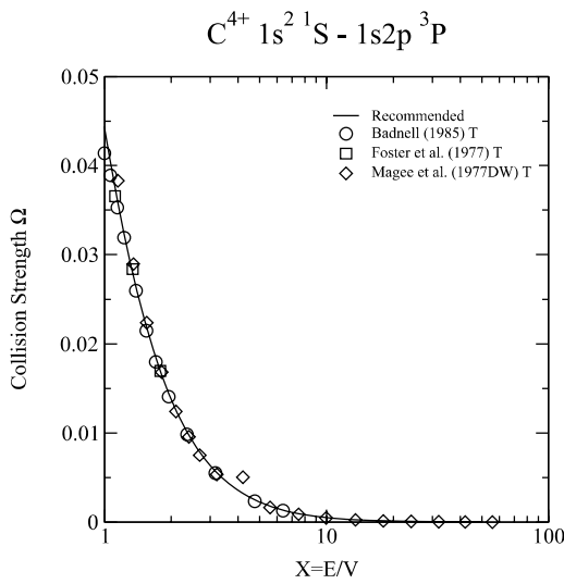
Graph 21: Collision strength for electron-impact excitation.
