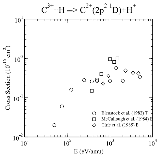
Graph 171: Cross section for charge exchange.
