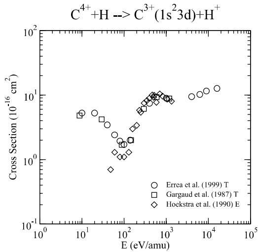
Graph 163: Cross section for charge exchange.
