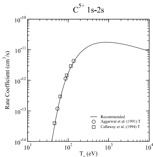
Graph 2: Rate coefficient for electron-impact excitation.
