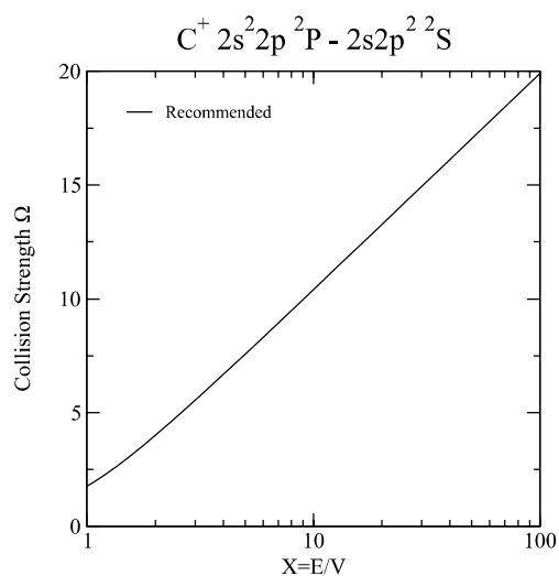
Graph 97: Collision strength for electron-impact excitation.
