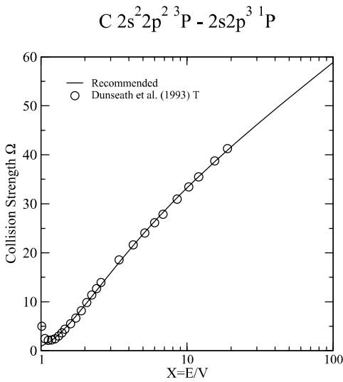
Graph 117: Collision strength for electron-impact excitation.
