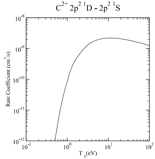
Graph 92: Rate coefficient for electron-impact excitation.
