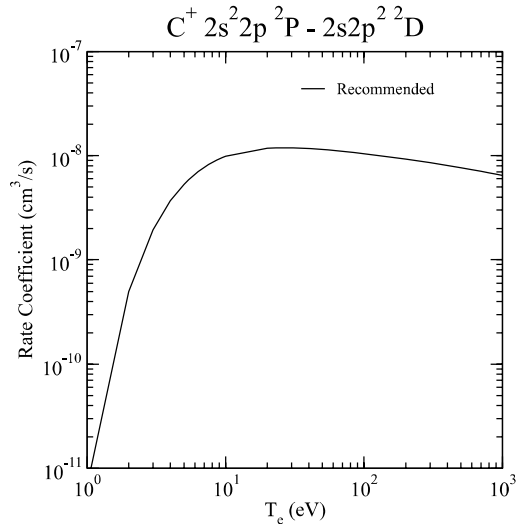
Graph 96: Rate coefficient for electron-impact excitation.
