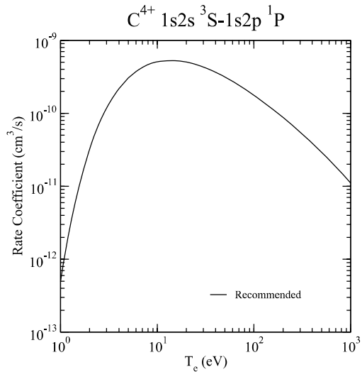
Graph 34: Rate coefficient for electron-impact excitation.
