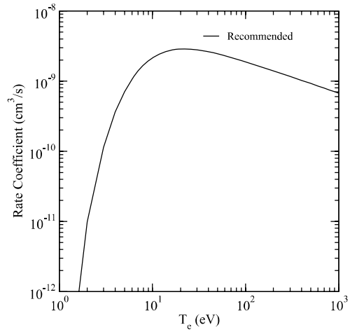
Graph 104: Rate coefficient for electron-impact excitation.
