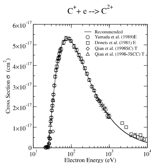
Graph 134: Same as previous Graph, but with the linear scale for the vertical axis.
