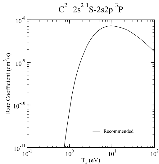
Graph 62: Rate coefficient for electron-impact excitation.
