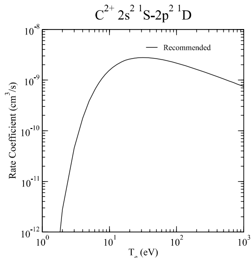
Graph 68: Rate coefficient for electron-impact excitation.
