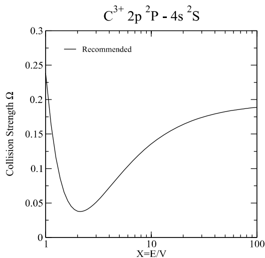
Graph 59: Collision strength for electron-impact excitation.
