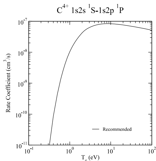
Graph 40: Rate coefficient for electron-impact excitation.
