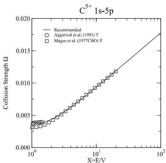
Graph 15: Collision strength for electron-impact excitation.
