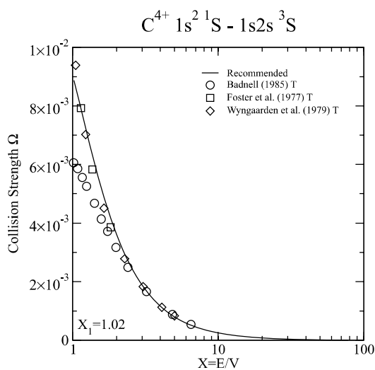
Graph 17: Collision strength for electron-impact excitation.
