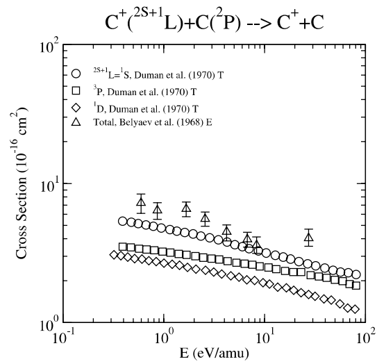
Graph 175: Cross section for charge exchange.
