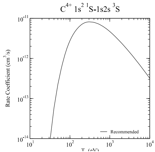
Graph 18: Rate coefficient for electron-impact excitation.
