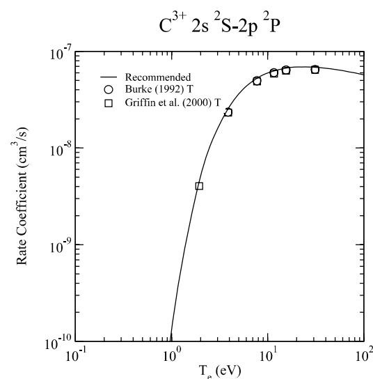
Graph 46: Rate coefficient for electron-impact excitation.
