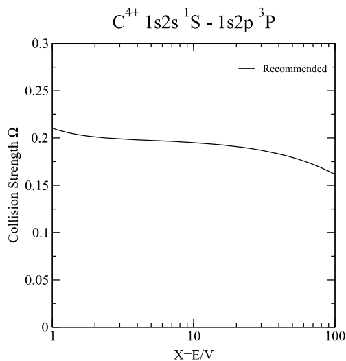
Graph 37: Collision strength for electron-impact excitation.
