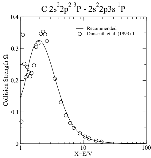
Graph 115: Collision strength for electron-impact excitation.
