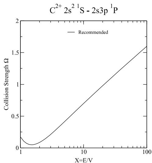
Graph 73: Collision strength for electron-impact excitation.
