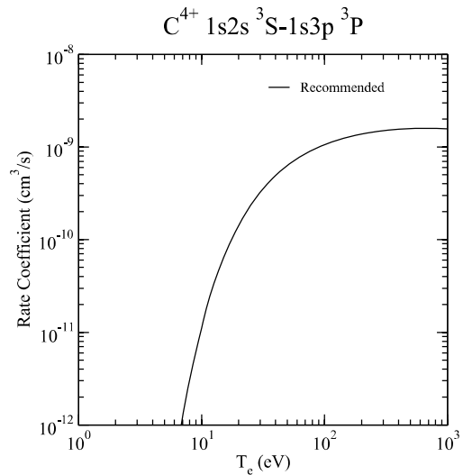
Graph 36: Rate coefficient for electron-impact excitation.
