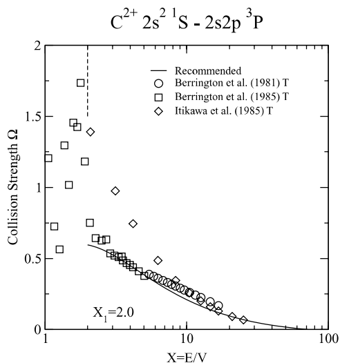
Graph 61: Collision strength for electron-impact excitation.
