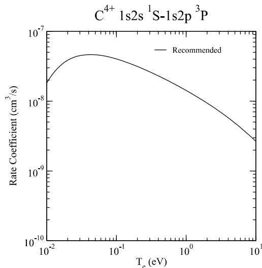
Graph 38: Rate coefficient for electron-impact excitation.
