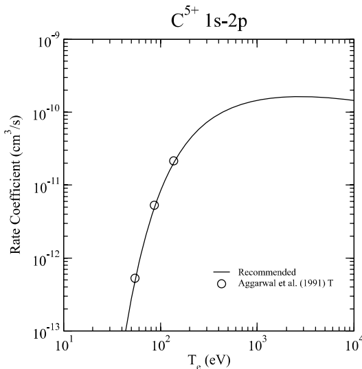
Graph 4: Rate coefficient for electron-impact excitation.
