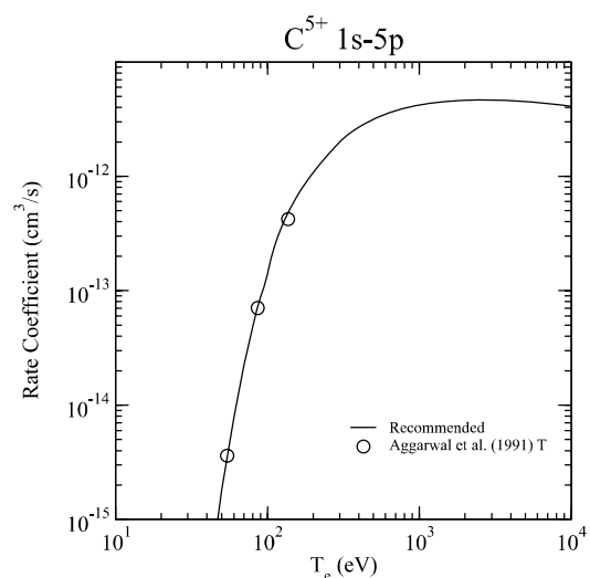
Graph 16: Rate coefficient for electron-impact excitation.
