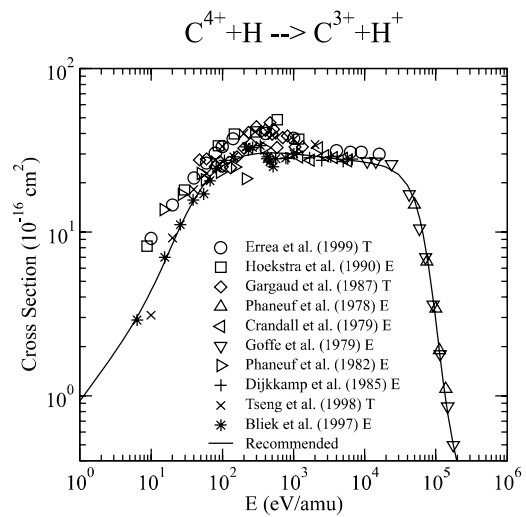
Graph 168: Cross section for charge exchange.
