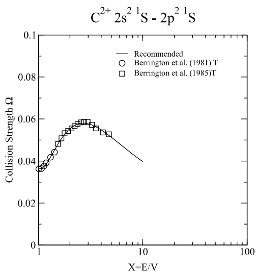
Graph 69: Collision strength for electron-impact excitation.
