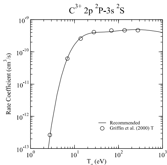
Graph 56: Rate coefficient for electron-impact excitation.
