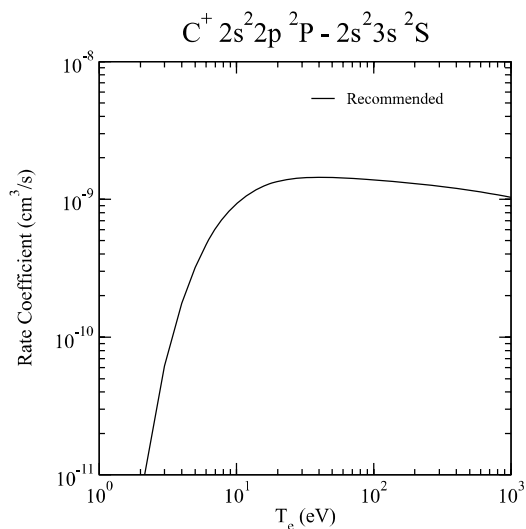
Graph 102: Rate coefficient for electron-impact excitation.
