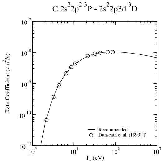
Graph 122: Rate coefficient for electron-impact excitation.
