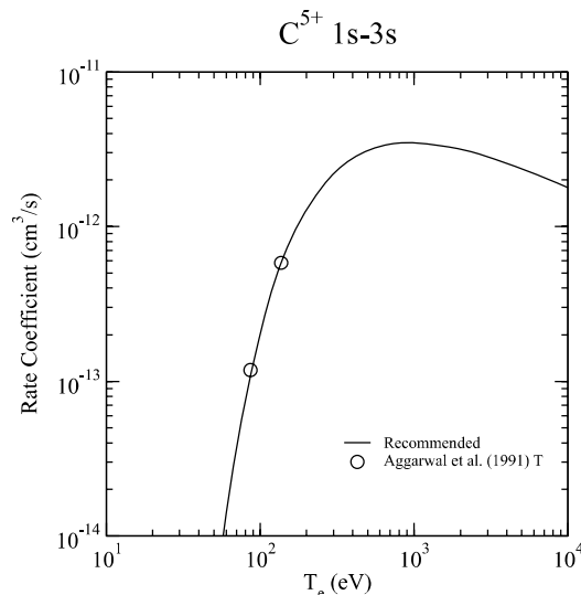
Graph 6: Rate coefficient for electron-impact excitation.
