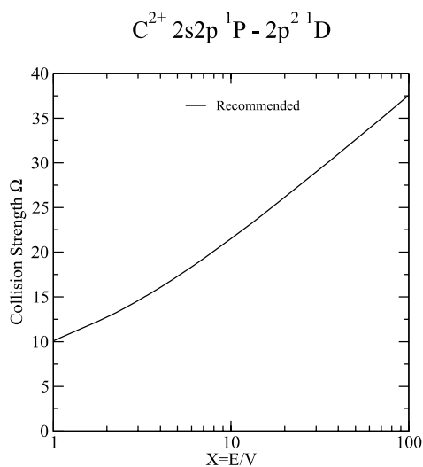
Graph 83: Collision strength for electron-impact excitation.
