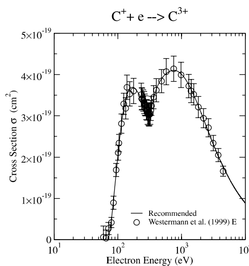
Graph 136: Same as previous Graph, but with the linear scale for the vertical axis.
