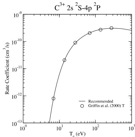
Graph 54: Rate coefficient for electron-impact excitation.
