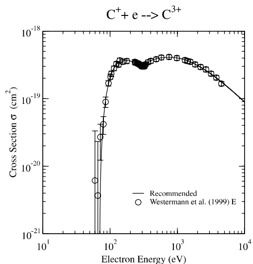
Graph 135: Cross section for electron-impact ionization.
