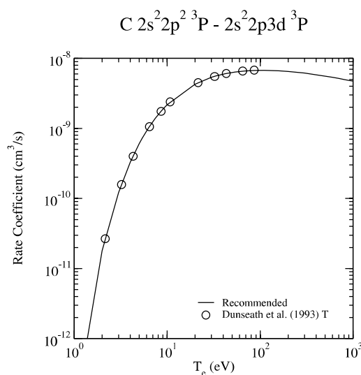
Graph 124: Rate coefficient for electron-impact excitation.
