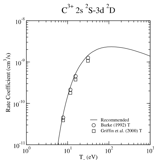
Graph 52: Rate coefficient for electron-impact excitation.
