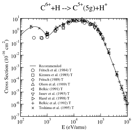
Graph 156: Cross section for charge exchange.
