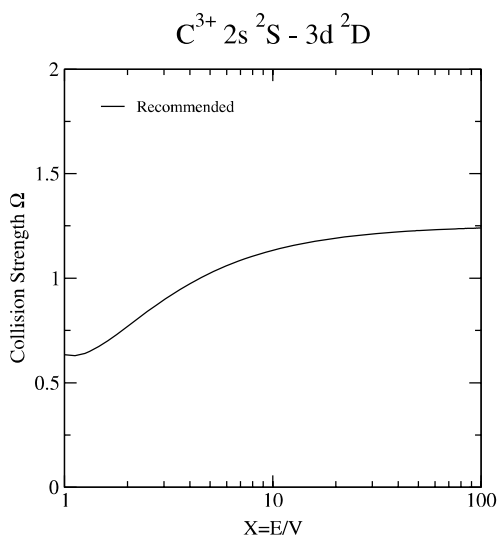
Graph 51: Collision strength for electron-impact excitation.
