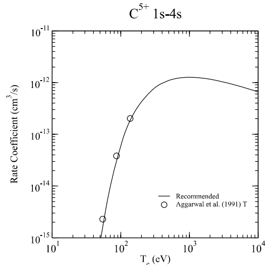
Graph 12: Rate coefficient for electron-impact excitation.
