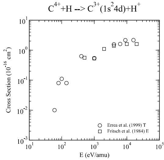
Graph 166: Cross section for charge exchange.
