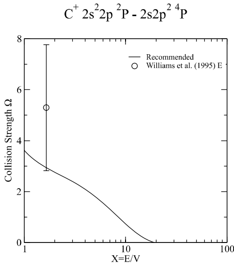
Graph 93: Collision strength for electron-impact excitation.
