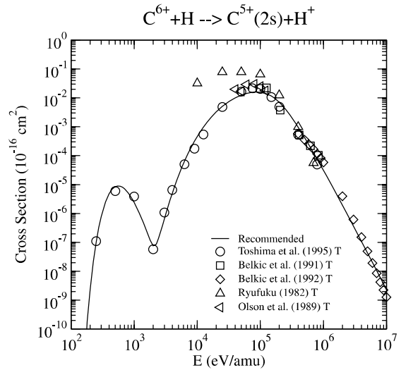
Graph 140: Cross section for charge exchange.
