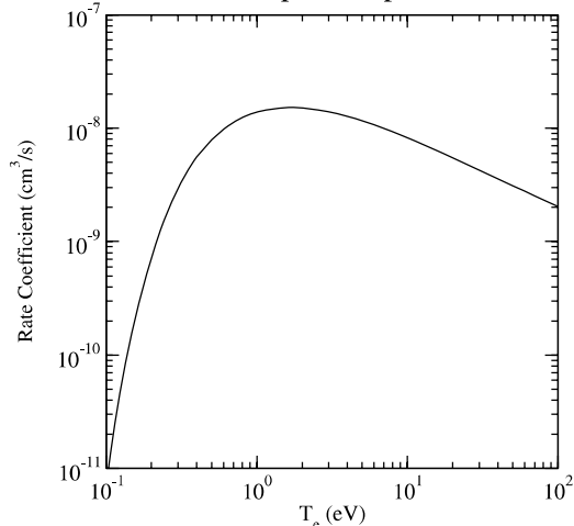
Graph 88: Rate coefficient for electron-impact excitation.
