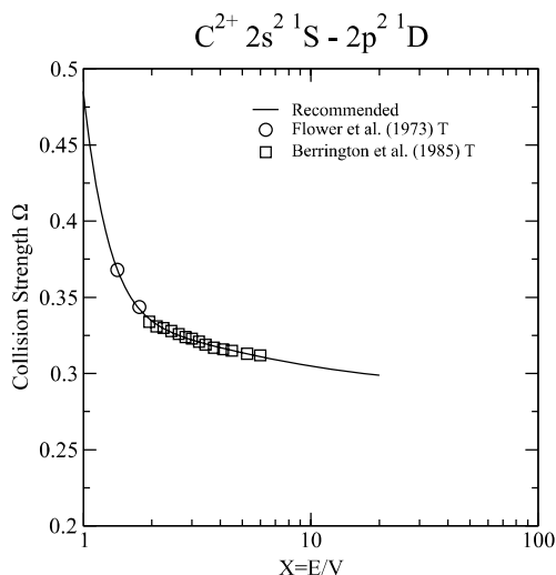
Graph 67: Collision strength for electron-impact excitation.
