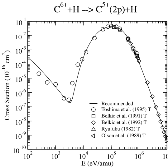
Graph 141: Cross section for charge exchange.
