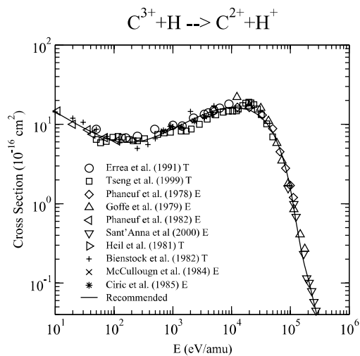
Graph 172: Cross section for charge exchange.
