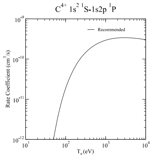
Graph 24: Rate coefficient for electron-impact excitation.
