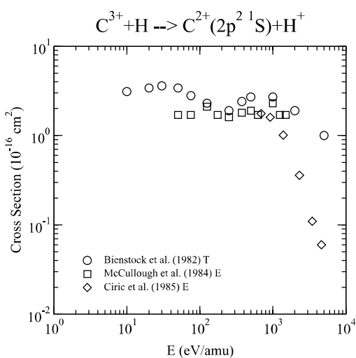
Graph 170: Cross section for charge exchange.
