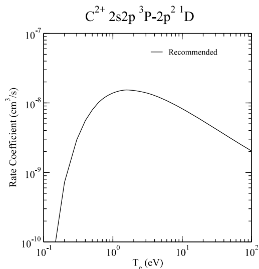
Graph 78: Rate coefficient for electron-impact excitation.
