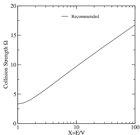
Graph 85: Collision strength for electron-impact excitation.
