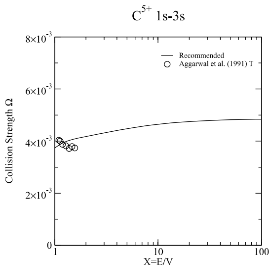
Graph 5: Collision strength for electron-impact excitation.
