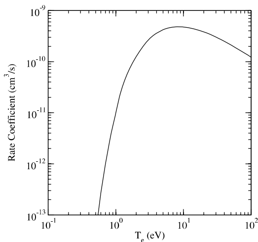
Graph 90: Rate coefficient for electron-impact excitation.
