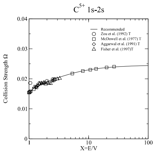
Graph 1: Collision strength for electron-impact excitation.
