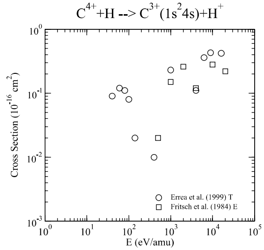
Graph 164: Cross section for charge exchange.
