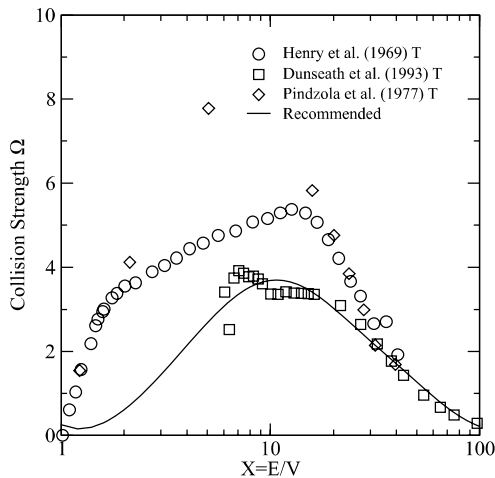
Graph 107: Collision strength for electron-impact excitation.
