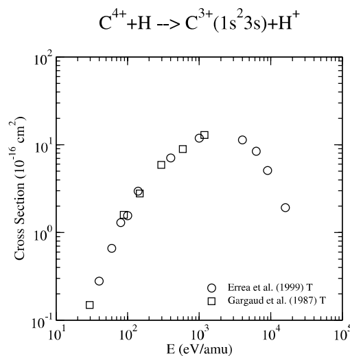
Graph 161: Cross section for charge exchange.
