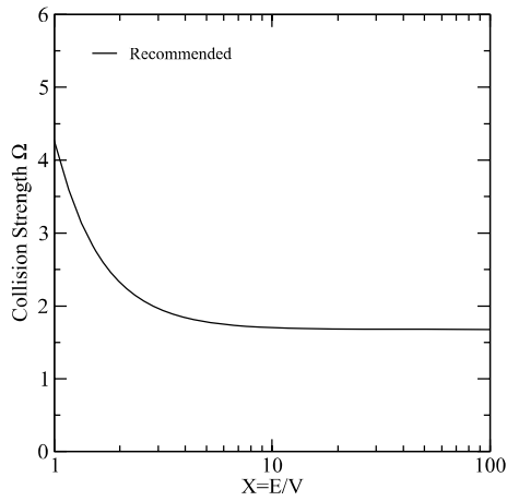
Graph 103: Collision strength for electron-impact excitation.
