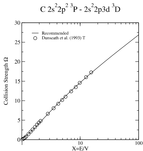
Graph 121: Collision strength for electron-impact excitation.
