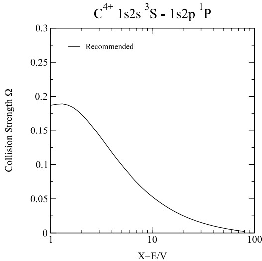
Graph 33: Collision strength for electron-impact excitation.
