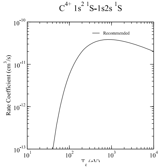
Graph 20: Rate coefficient for electron-impact excitation.
