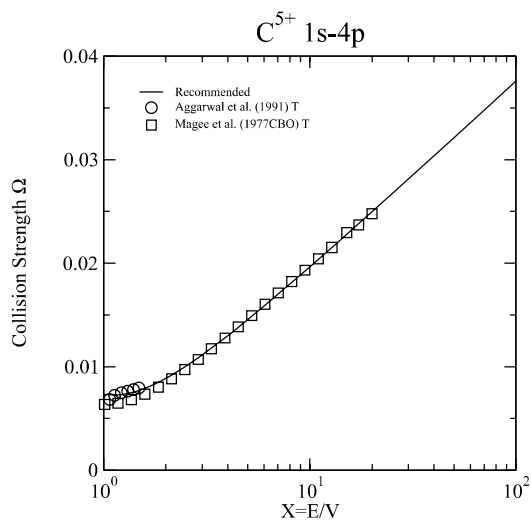
Graph 13: Collision strength for electron-impact excitation.
