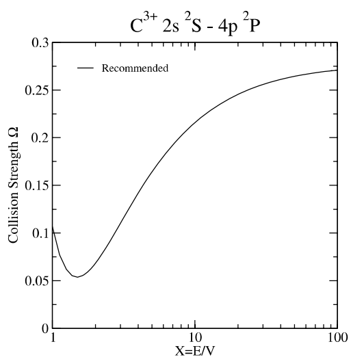
Graph 53: Collision strength for electron-impact excitation.
