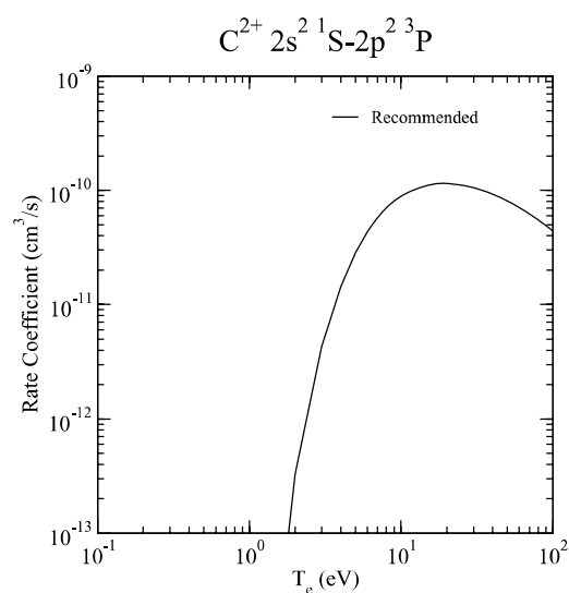
Graph 66: Rate coefficient for electron-impact excitation.
