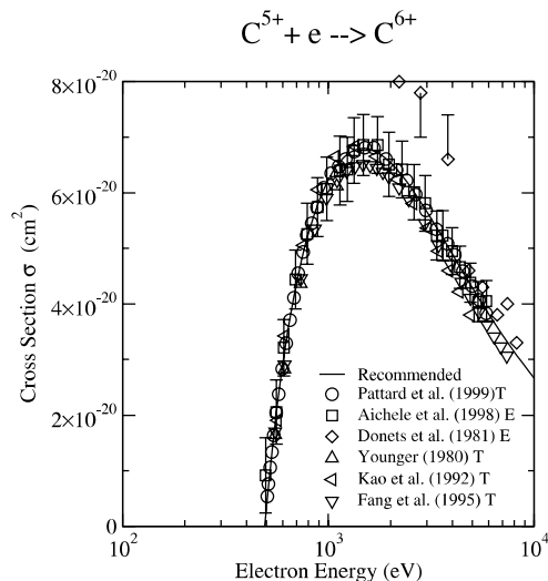
Graph 126: Same as previous Graph, but with the linear scale for the vertical axis.
