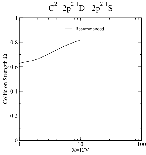
Graph 91: Collision strength for electron-impact excitation.
