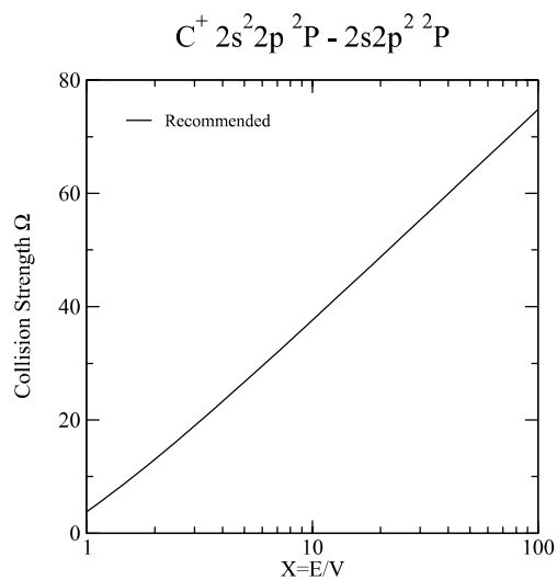
Graph 99: Collision strength for electron-impact excitation.
