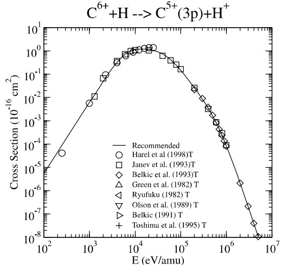
Graph 144: Cross section for charge exchange.
