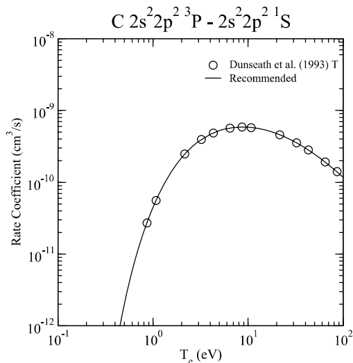
Graph 110: Rate coefficient for electron-impact excitation.
