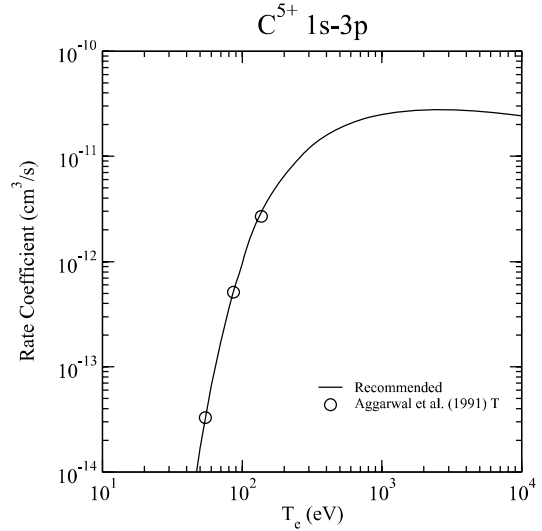
Graph 8: Rate coefficient for electron-impact excitation.
