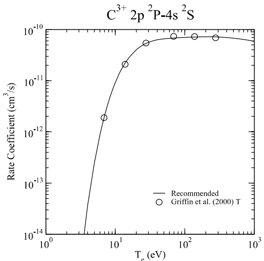
Graph 60: Rate coefficient for electron-impact excitation.
