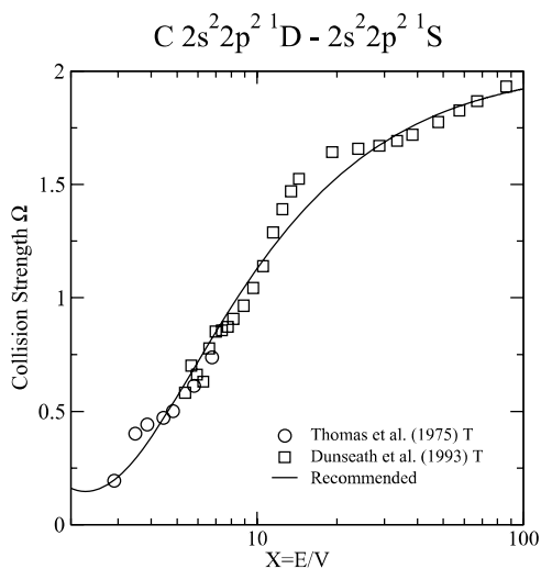
Graph 111: Collision strength for electron-impact excitation.
