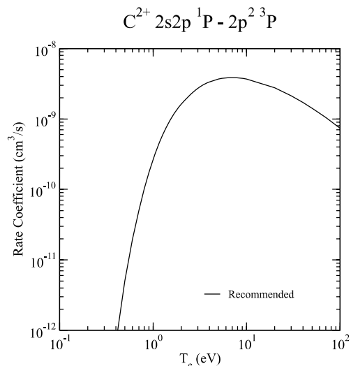
Graph 82: Rate coefficient for electron-impact excitation.
