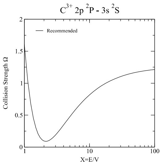
Graph 55: Collision strength for electron-impact excitation.
