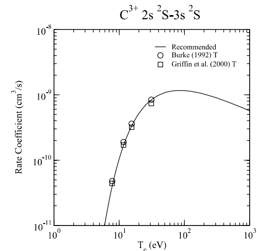
Graph 48: Rate coefficient for electron-impact excitation.
