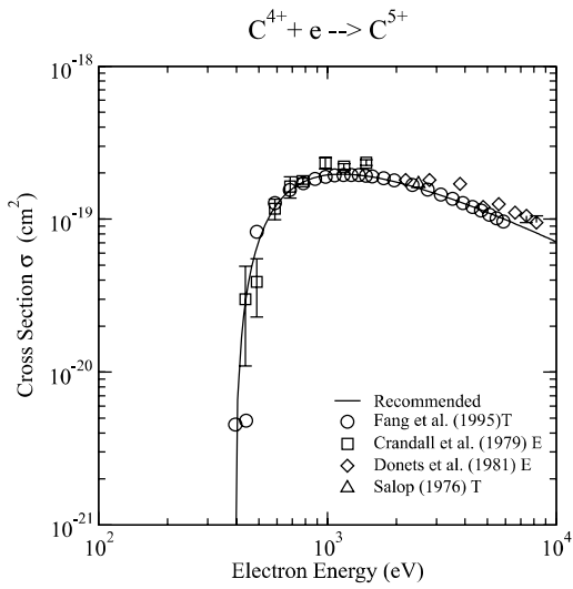
Graph 127: Cross section for electron-impact ionization.
