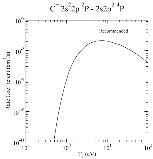
Graph 94: Rate coefficient for electron-impact excitation.
