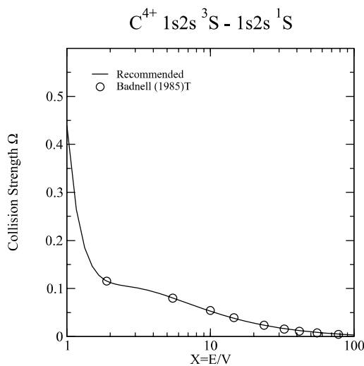
Graph 29: Collision strength for electron-impact excitation.
