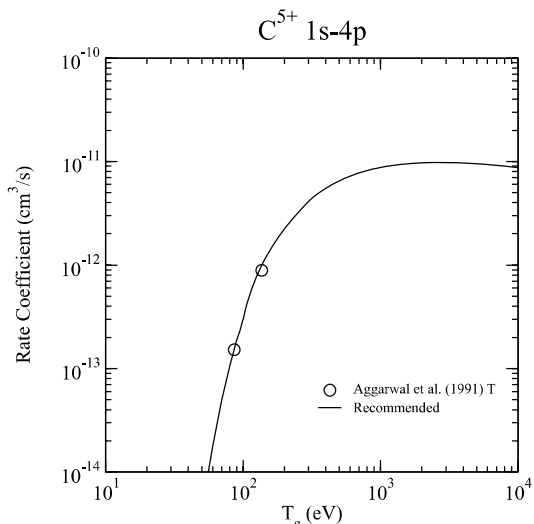
Graph 14: Rate coefficient for electron-impact excitation.
