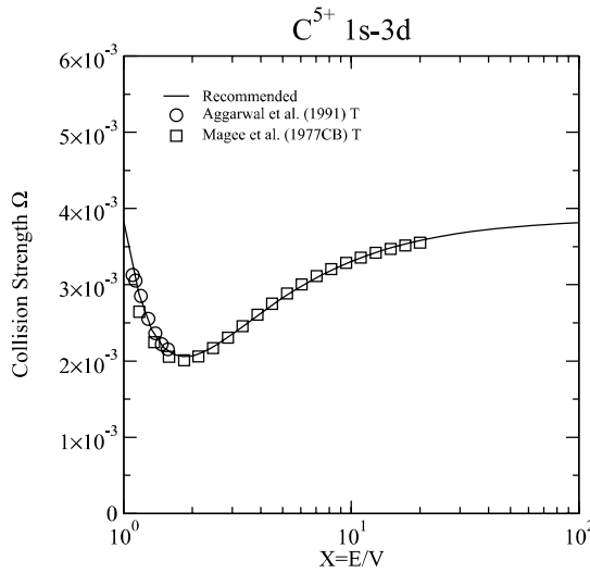
Graph 9: Collision strength for electron-impact excitation.
