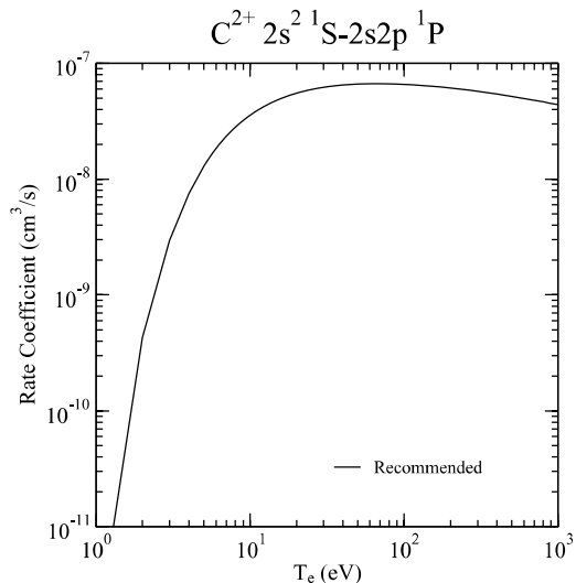
Graph 64: Rate coefficient for electron-impact excitation.
